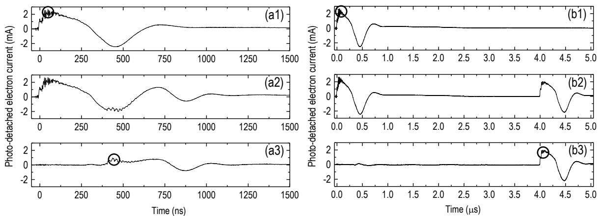
Figure 3. (a1) Single-laser photo-detachment signal. (a2) Double-laser photo-detachment signal, with \Delta t = 400 ns. (a3) Subtraction signal, i.e., (a2 – a1). (b1) to (b3) Similar, with \Delta t = 4 \mu s. The inset circles define the amplitudes used for the calculation of the n_{\bar{e}}^- / n_0^- ratio. Operating conditions: H 2 ; 600 W.
