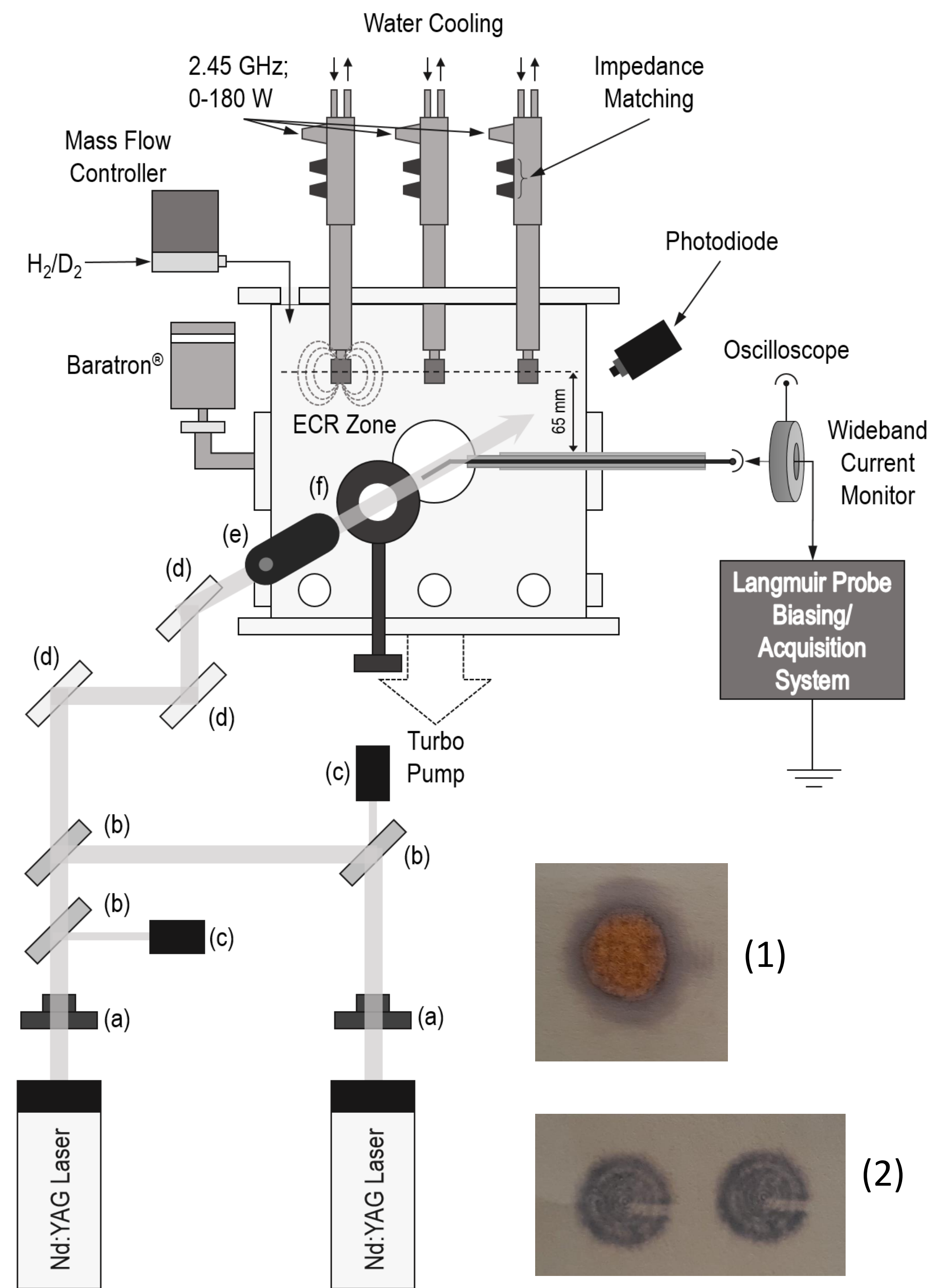
(a) \frac{1}{2} wave-plate on a rotation mount; (b) beam splitters; (c) beam dumps; (d) mirrors; (e) expander with \varnothing 2.5 mm and \varnothing 5 mm diaphragms; (f) pyroelectric laser beam energy sensor; (1) burn pattern of the verifying the concentric alignment of the two separate laser beams; (2) the corresponding burn pattern of the alignment of the two beams with the electrostatic probe used for measurements
