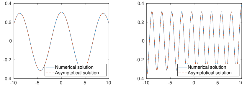
Fig. 1.3 Eigenfunctions \varphi_5 (left plot) and \varphi_{20} (right plot). \beta = 0.1 .
