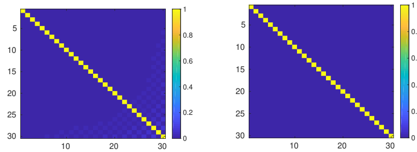
Fig. 1.4 Inner product matrices for solutions: asymptotic (left plot) and numerical (right plot). \beta = 0.1 .
