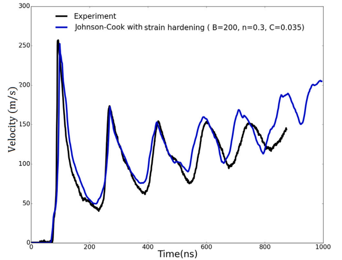
Fig. 8. Calculated and analyzed rear free-velocity profiles for pure aluminum using Johnson–Cook with strain hardening model.
