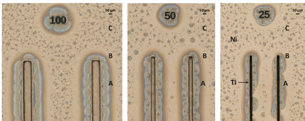
FIGURE 3 Top view images of the wafer surface showing trenches of different widths after etching: 100\ \mu\text{m} (left), 50\ \mu\text{m} (middle) and 25\ \mu\text{m} wide trenches
