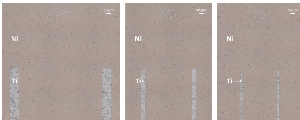
FIGURE 2 Top view images of the wafer surface showing trenches of different widths before etching: 100\ \mu\text{m} (left), 50\ \mu\text{m} (middle) and 25\ \mu\text{m} wide trenches
