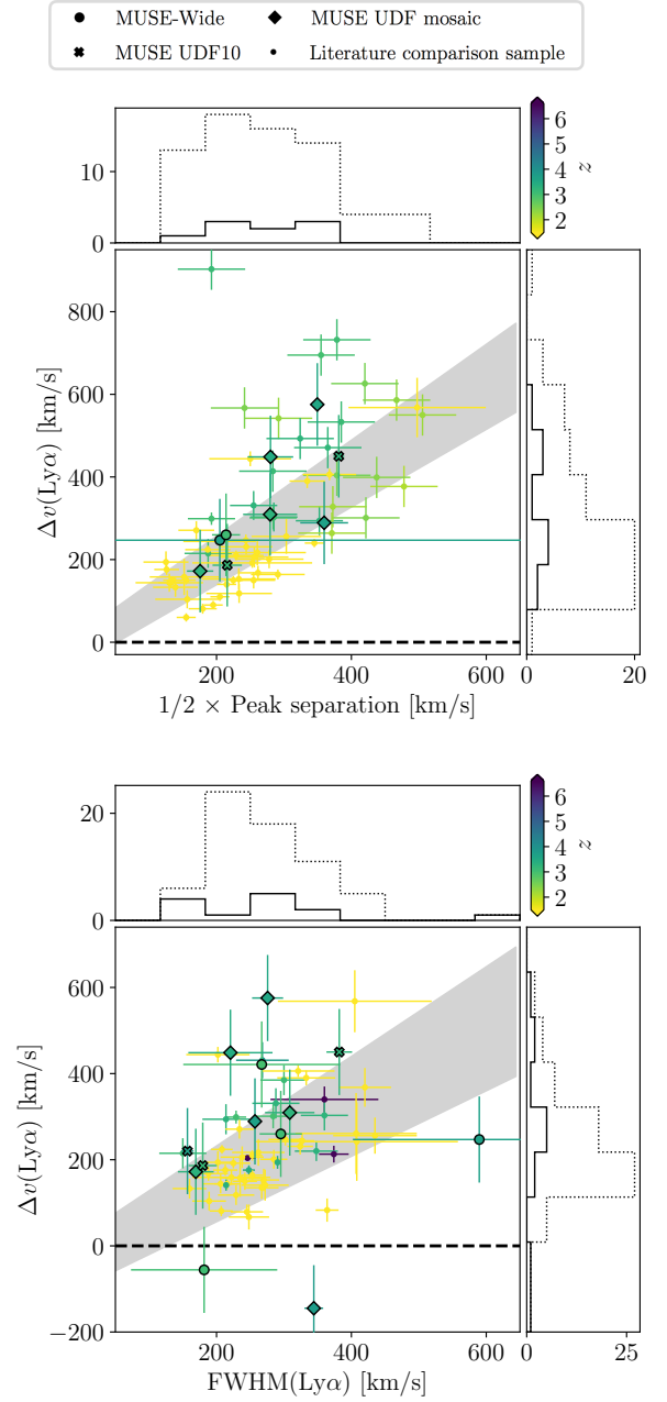
Fig. 15. Comparison of the velocity offset of \text{Ly}\alpha and half the \text{Ly}\alpha peak separation for objects with \text{Ly}\alpha line profiles containing both a red peak and a blue bump ( top ) and the \text{Ly}\alpha FWHM ( bottom ). These are the quantities used to predict \Delta v_{\text{Ly}\alpha} ( Verhamme et al. 2018 approx.) on the x -axis in Fig. 14. The gray bands show the empirical relations presented by Verhamme et al. (2018) . The small dots present a collection of literature measurements from Kulas et al. (2012) , Leitet et al. (2013) , Oesch et al. (2015) , Hashimoto et al. (2015) , Henry et al. (2015) , Guaita et al. (2016) , Izotov et al. (2016a,b) , Stark et al. (2017) , Verhamme et al. (2017, 2018) , Yang et al. (2017) , Matthee et al. (2020b) , Muzahid et al. (2020) , and Matthee et al. (2021) . All points are color coded according to object redshift. The solid histograms show the measurements presented in this study, whereas the dotted histograms include the measurements from the literature.
