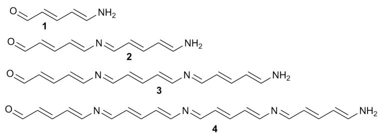
Chart 1. 1,6-Polyazaacetylene monomer ( 1 ) and respective oligomers ( 2–4 ): all-trans model structures.
