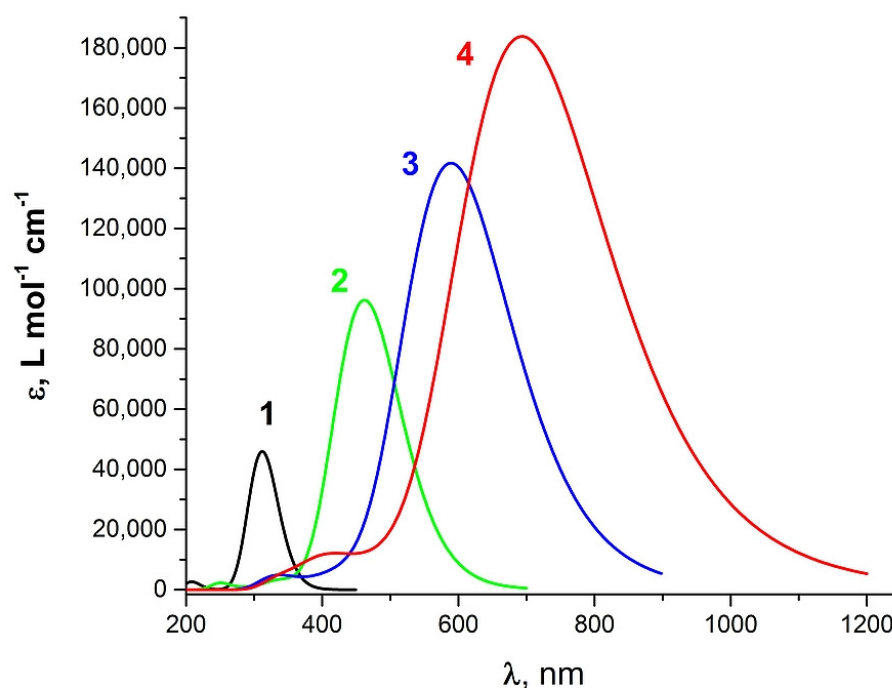
Figure 3. Calculated (B3LYP/aug-cc-pVDZ//B3LYP/aug-cc-pVDZ model chemistry) absorption spectra of molecules 1–4 (Chart 1) in dichloromethane; TD-SCF was solved for 10 states.
