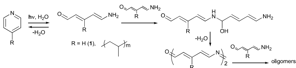
Scheme 1. Photoinduced pyridine ring-opening and subsequent polycondensation.
