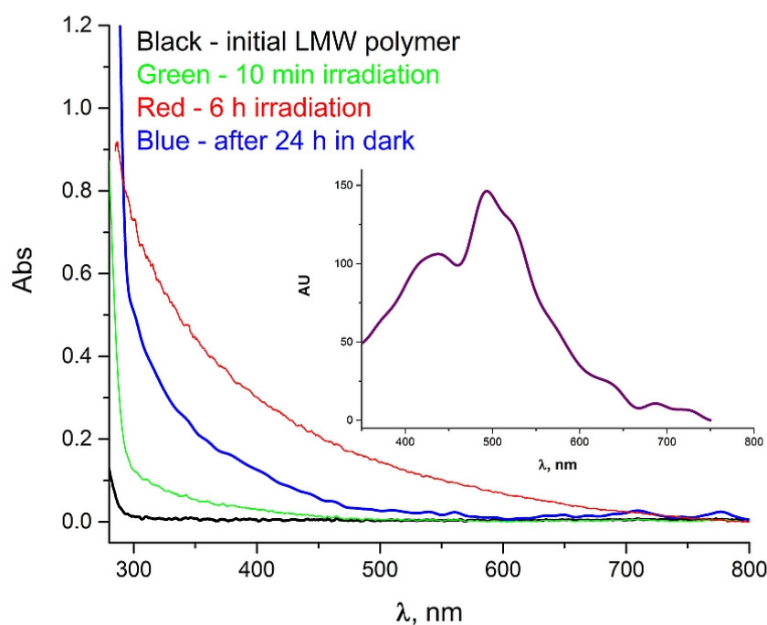
Figure 1. UV-Vis spectra of low-MW P4VP/Py gel samples in methylene chloride before and after irradiation at 312 nm as well as after holding the 6 h irradiated sample in the dark for 24 h. Inset: fluorescence spectrum of a thin film of a sample irradiated for 6 h (excitation at 350 nm).
