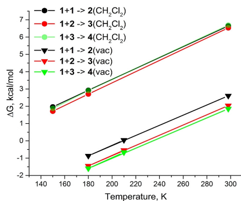
Figure 4. Calculated \Delta G of the proposed polycondensation reactions in dichloromethane and in vacuum.
