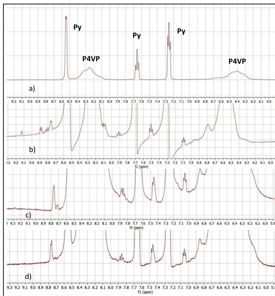
Figure 2. (a) 1 H NMR spectrum of P4VP/Py gel before irradiation; (b) after 1 h irradiation of P4VP/Py gel at 312 nm; (c) after 6 h irradiation at 312 nm; (d) after 6 h irradiation of P4VP/Py gel and subsequent 24 h storage in the dark.
