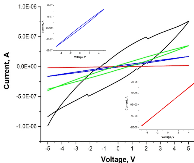
Figure 6. Current–voltage curves of low-MW P4VP/Py gel sample (thickness 230 mm, cross-section 5 \times 5 mm) before irradiation (black curve); after irradiation at 254 nm for one hour and 10 h holding in the dark (green curve); after additional one-hour irradiation and holding the sample in the dark for 10 h (blue curve and upper inset); after the third one-hour irradiation and holding the sample in the dark for 10 h (red curve and lower inset). The sweep rate was 1.7 V/s.
