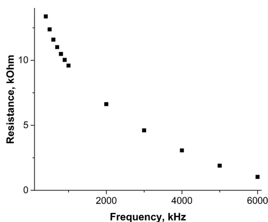
Figure 5. Resistance dependence on the AC voltage frequency of the low-MW gel. Voltage amplitude 35 mV, thickness of the sample 230 \mu\text{m} , cross-section 5 \times 5 mm.
