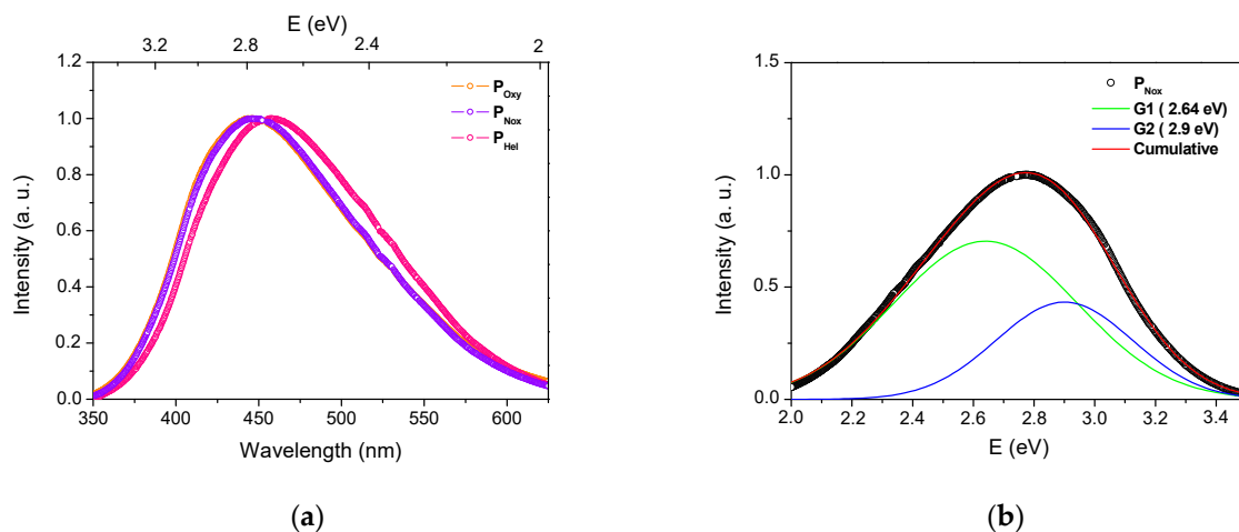
Figure 3. (a) Normalized PL spectra of the three Ce-doped preforms under excitation at 320 nm. (b) PL spectrum Gaussian shape decomposition for the P Nox sample.
