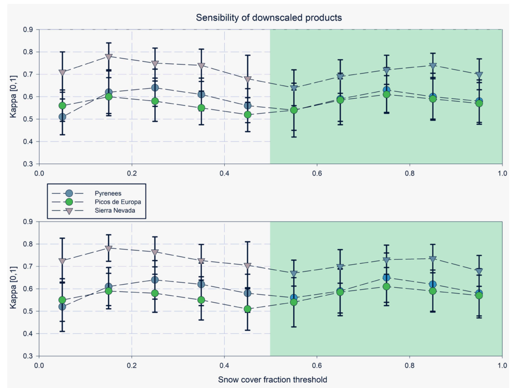
Figure 5. The mean value and standard deviation of the Kappa coefficients obtained in the paired sensitivity test to determine the upper and lower FSC thresholds. The upper graph depicts the ProbMODIS sensitivity test, and the lower graph shows the ProbSentinel sensitivity test. The light green shaded area shows the results for the upper limit sensitivity tests, and the non-shaded area the results of the lower limit sensitivity test. These graphs include the results obtained in the three test areas.
