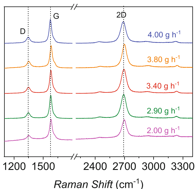
Fig. 10. Raman spectrum of samples synthesized through the plasmas process described in the current research.
