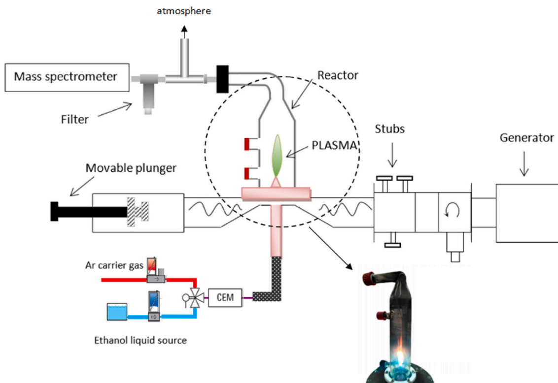
Fig. 1. Schematic drawing of the experimental set up (no to scale).
