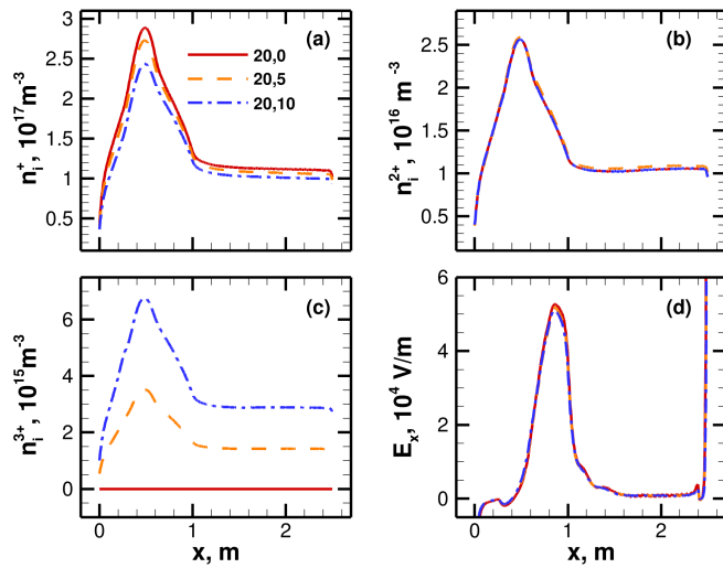
FIG. 3: Spatially and temporally averaged plasma properties. All quantities are averaged in y direction and over 5 \mu\text{s} period in steady state. (a) \text{Xe}^+ density, (b) \text{Xe}^{2+} density, (c) \text{Xe}^{3+} density, and (d) axial electric field. All the physical and numerical parameters are fixed while \alpha_d = 20\% and \alpha_t is varied. Three cases corresponding to \alpha_t = 0, 5 and 10\% are shown.
