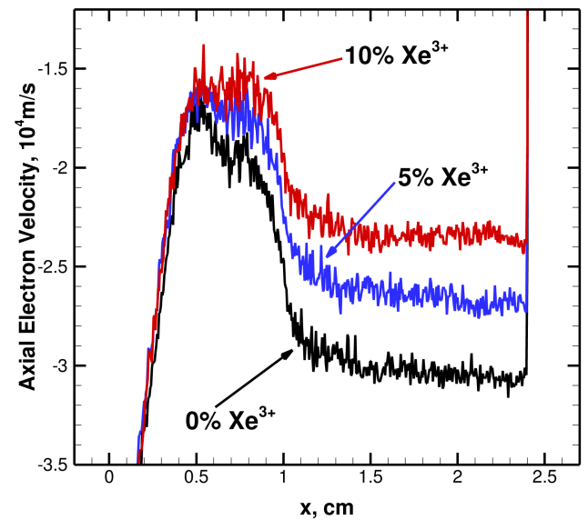
FIG. 4: Cross-field electron transport is reduced when increasing triply charged ion species fraction. Plasma properties are averaged in y direction and over 5 \mu\text{s} from t = 15 \mu\text{s} - 20 \mu\text{s} . For all cases, \alpha_d = 20\% is used and the results for \alpha_t = 0, 5\% , and 10\% are shown.
