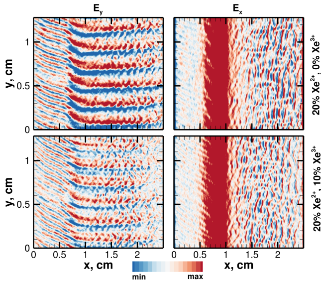
FIG. 1: Effect of increasing triply charged ion concentration on instantaneous azimuthal ( E_y ) and axial ( E_x ) electric field due to coupling between ECDI and IITSI. Top row: \alpha_d = 20\% and \alpha_t = 0 ; bottom row: \alpha_d = 20\% and \alpha_t = 10\% . Results are shown for t = 18 \mu\text{s} , i.e., after the steady state is reached. The colorbar is saturated for better visualization of axial fluctuations in the downstream region, where min and max on the color scale correspond to -2.0 \times 10^4 \text{ V/m} and 2.0 \times 10^4 \text{ V/m} , respectively.
