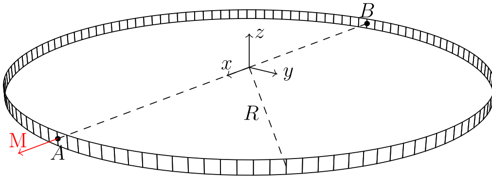
FIGURE 9 Deployable ring subjected to a torsion moment.
