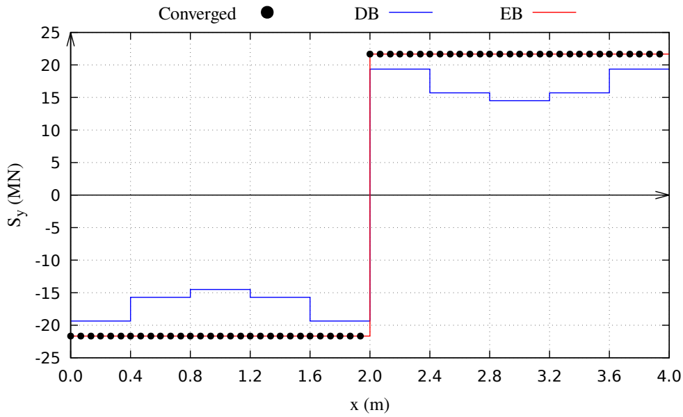
(a) Shear force diagram
