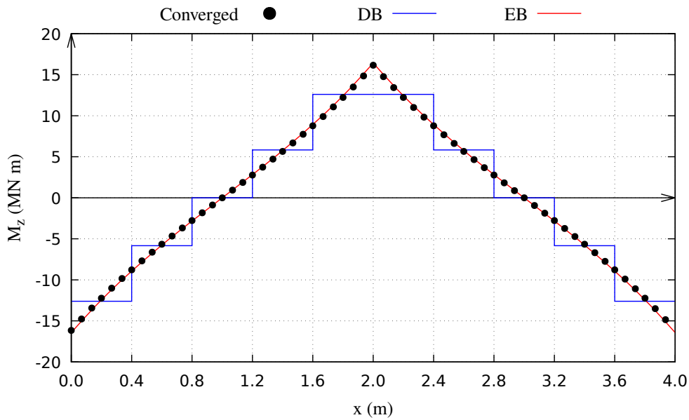
(b) Bending moment diagram
