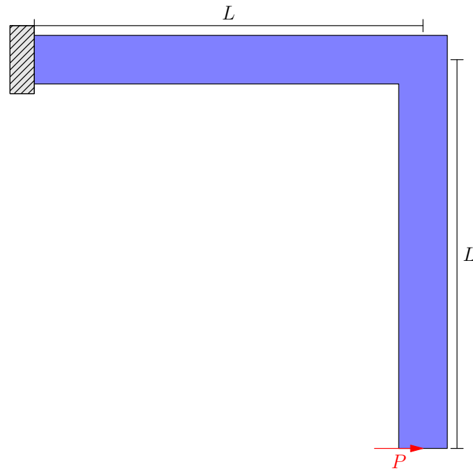
FIGURE 7 L-shaped frame subjected to a tip force.
