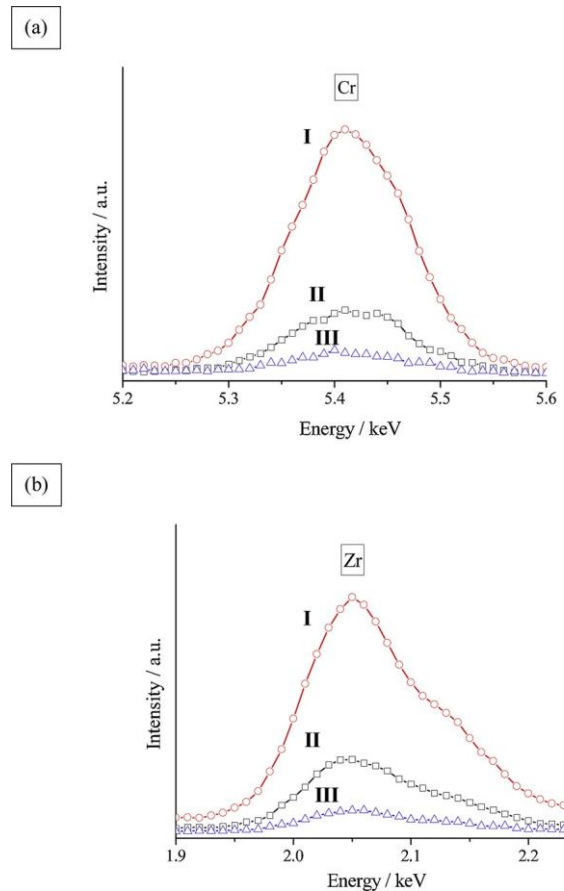
Fig. 4. EDS peaks for zirconium and chromium at spots I, II and III corresponding to over an irregular-shaped deposit, the grain boundary \beta phase and the \alpha matrix, respectively, shown in Fig. 3b.
