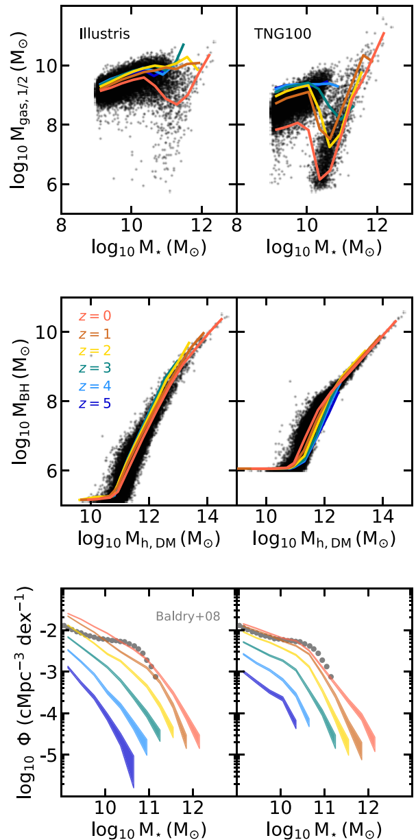
Figure 10. Different diagnostics to understand the evolution of the overall normalization of the M_{\text{BH}} - M_{\star} mean relation with time. Top panels: Mean mass of the gas contained in the half-mass radius of the galaxies; the entire population at z = 0 is shown in black. The gas content in the inner region of the galaxies diminishes with time. Middle panels: Mean BH mass as a function of the dark matter mass of their host haloes. We show in black all the haloes with BHs at z = 0 . At fixed dark matter halo mass, we find a larger evolution in TNG100, and almost no evolution in Illustris. Bottom panels: Galaxy stellar mass functions. Grey symbols show the observational constraints of Baldry, Glazebrook & Driver (2008) ( z \sim 0 ). The low-mass end of the galaxy mass function is overestimated in Illustris ( M_{\star} \leq 10^{10.5} M_{\odot} ); a better agreement is found for TNG100.
