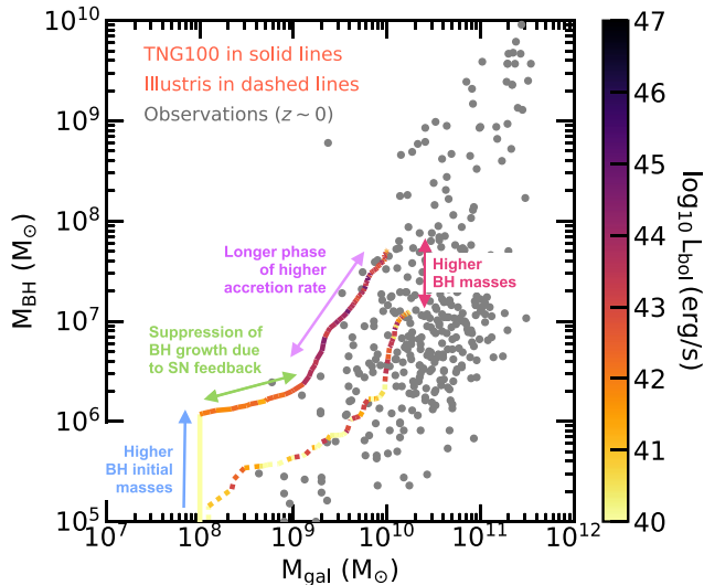
Figure 9. Illustration of one set of matched galaxies in TNG (solid line) and Illustris (dashed line) with total stellar mass of M_{\star} = 10^{10} M_{\odot} at z = 0 . Not all BHs in the same galaxy mass range follow the same track, but at least a large fraction does so. The BHs in TNG start with a higher initial mass, are stunted by an efficient SN feedback, experience longer phases of higher accretion rate than the BHs in Illustris. Consequently, the BHs in TNG reach larger masses by z = 0 in galaxies with M_{\star, z=0} = 10^{10} M_{\odot} . A few examples for galaxies of M_{\star, z=0} = 10^{10} M_{\odot} and M_{\star, z=0} = 10^{11} M_{\odot} are given in Appendix D.
