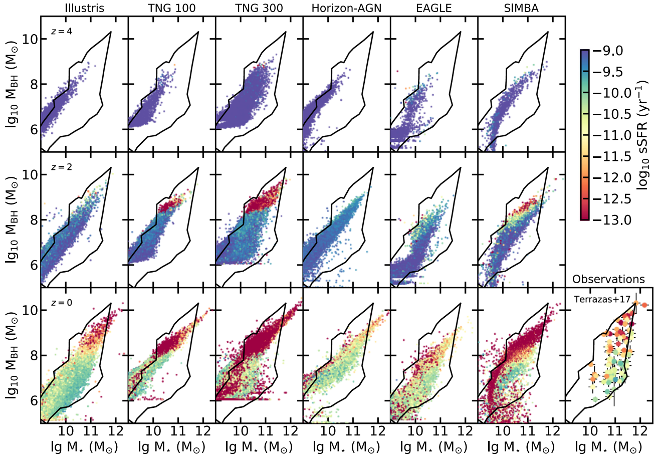
Figure B1. M_{\text{BH}} - M_{\star} diagram at z = 4, 2, 0 for all the simulations. We colour-code the simulated BHs with the specific star formation rate (sSFR) of their host galaxies. We set \text{sSFR} = 10^{-13} \text{ yr}^{-1} for galaxies with lower sSFR. The limit \text{sSFR} = 10^{-11} \text{ yr}^{-1} is often used to define star-forming galaxies (with higher sSFR) or quiescent galaxies (with lower sSFR). In the figure, galaxies with blue colours are forming stars, and yellow to red galaxies are quiescent. We show in the last right-hand panel the observed star-forming and quiescent galaxies of Terrazas et al. (2017) for references, colour-coded by their sSFR as well. To guide the eye, we again reproduce the black region representing the observational sample of Reines & Volonteri (2015) at z = 0 in each panel.
