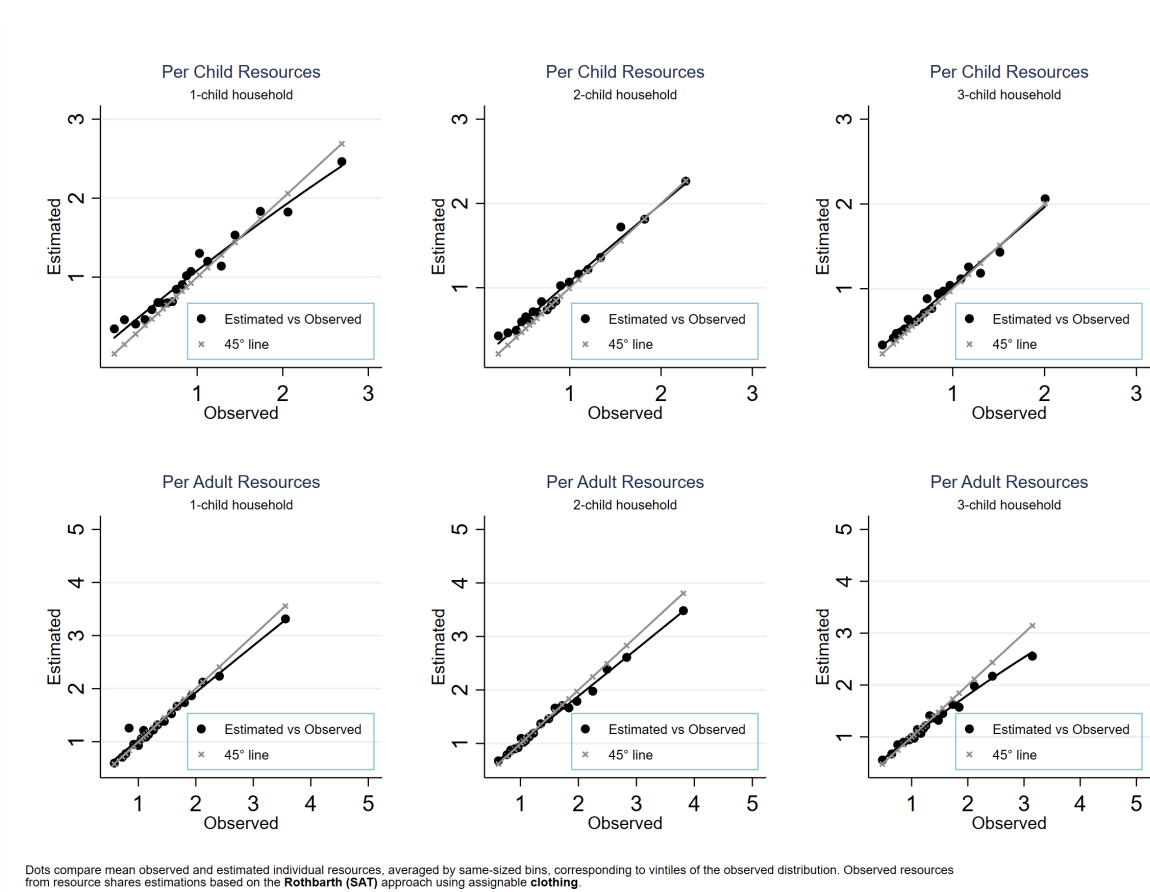
Figure 4: Observed vs. Estimated Resources (Equal-Size Bins): Rothbarth Approach
