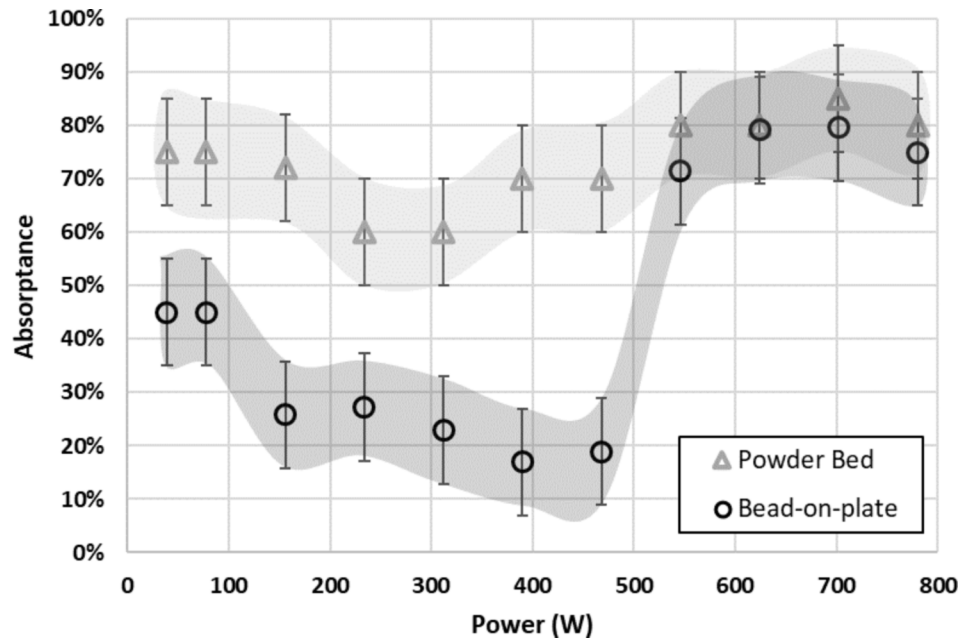
Fig. 7. Measured absorptance versus laser power for single tracks carried out on powder beds (gray triangles) or bare substrates (black circles). V = 0.2 m/s, d = 180 µm (errors bars come from the reference absorptance value on aluminium \pm 10\% and the fluctuation of the absorptance vs time data).
