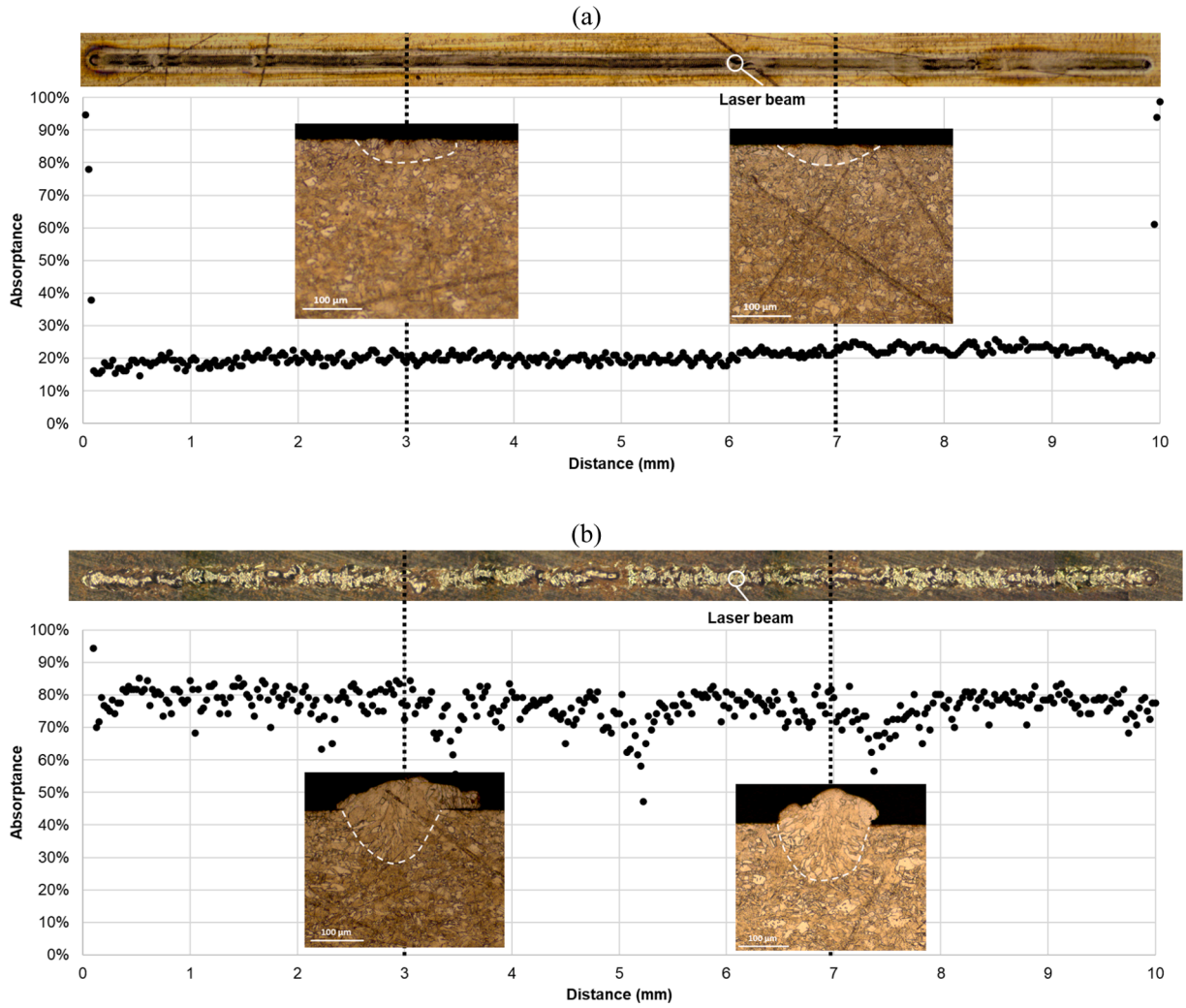
Fig. 5. Absorptivity measurement during (a) a single bead-on-plate fusion track, (b) a single L-PBF track ( P = 468 W, V = 0.5 m/s, d = 150 \mu m, VED = 53 J/mm 3 ).
