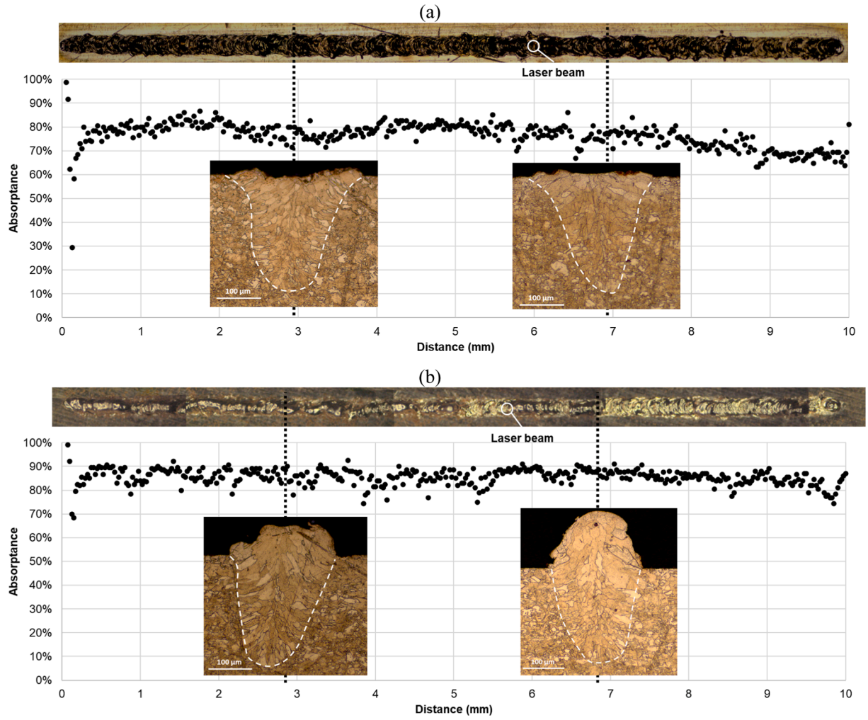
Fig. 6. Absorptivity measurement during (a) a single bead-on-plate fusion track, (b) a single L-PBF track ( P = 780 W, V = 0.5 m/s, d = 150 µm, VED = 88 J/mm 3 ).
