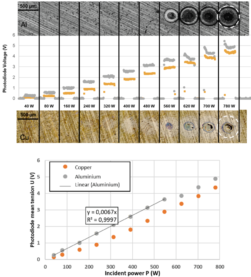
Fig. 4. Calibration of the photodiode signals for static laser shoots ( t_{\text{pulse}} = 20 ms) and incremental power values (laser spot in white dotted line): (a) experimental signals and corresponding surface aspects, (b) calibration curves (a nonmelt regime is shown up to 480 W on the two metals).
