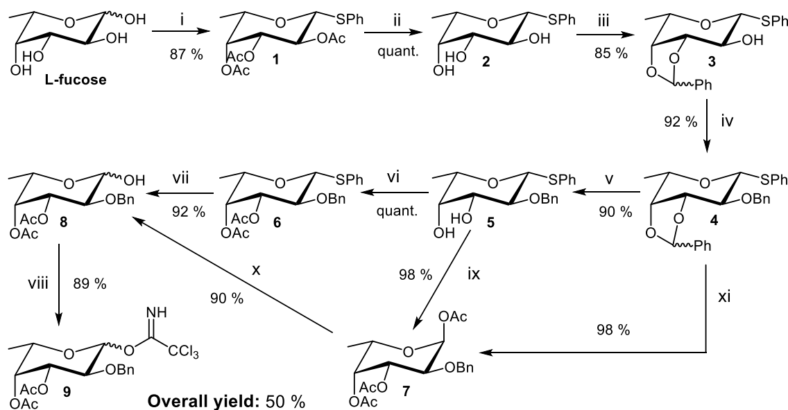
Scheme 2. Synthetic routes developed. Reagents and conditions: (i) Ac 2 O, BF 3 ·OEt 2 , rt, 10 min, then PhSH, rt, 4 h; (ii) NaOMe, MeOH, rt, 2 h; (iii) benzaldehyde dimethylacetal, p -TsOH, DMF, 50 °C, 1 h; (iv) BnBr, NaH, DMF, rt, 1 h; (v) aq. AcOH 80%, 80 °C, 1 h; (vi) Ac 2 O, Py, rt, 6 h; (vii) NBS, acetone, H 2 O, rt, 1 h; (viii) trichloroacetonitrile, DBU, CH 2 Cl 2 , rt, 16 h; (ix) Ac 2 O, I 2 , rt, 15 min; (x) hydrazine acetate, DMF, 50 °C, 30 min; (xi) Ac 2 O, HClO 4 -SiO 2 , rt, 1 h.
