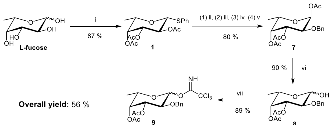
Scheme 3. Best synthetic approach developed without chromatographic purification of the intermediaries 3 and 4 . Reagents and conditions: (i) Ac 2 O, BF 3 ·OEt 2 , rt, 10 min, then PhSH, rt, 4 h; (ii) NaOMe, MeOH, rt, 2 h; (iii) benzaldehyde dimethylacetal, p -TsoH, DMF, 50 °C, 1 h; (iv) BnBr, NaH, DMF, rt, 1 h; (v) Ac 2 O, HClO 4 -SiO 2 , rt, 1 h; (vi) hydrazine acetate, DMF, 50 °C, 30 min; (vii) trichloroacetonitrile, DBU, CH 2 Cl 2 , rt, 16 h.
