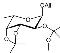
Fig. 2. Chemical structure of the 2- O -mixed acetal formed.
