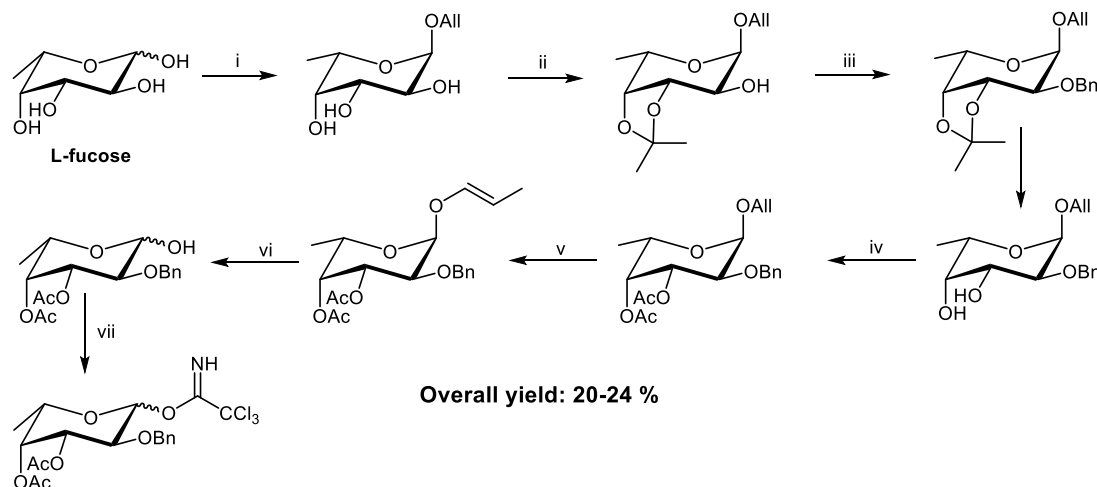
Scheme 1. Synthetic route reported in the literature. Variant A [lit. 5]. Reagents and conditions: (i) AlOH, H + , 98 °C, 8 h; (ii) acetone, TsOH, 56 °C, 4 h; (iii) BnBr, NaH, DMF, rt, 2 h; (iv) TFA 50%, CH 2 Cl 2 , rt, 16 h; (v) Ac 2 O, Py, rt, 16 h; (vi) (Ph 3 P) 3 RhCl, DBU, EtOH/H 2 O, 80 °C, 3 h; (vii) 1 N HCl, rt, 36 h; (viii) trichloroacetonitrile, DBU, CH 2 Cl 2 , rt, 90 min. Variant B [lit. 6]. Reagents and conditions: (i) AlOH, CSA, 90 °C, 2 h; (ii) 2,2-dimethoxypropane, acetone, CSA, rt, 24 h; (iii) BnBr, NaH, TBAI, THF/DMF, rt, 16 h; (iv) AcOH 70%, 45 °C, 4 h; (v) Ac 2 O, Et 3 N, DMAP, rt, 16 h; (vi) [Ir(COD)(PMePh 2 ) 2 ] + PF 6 - , H 2 , THF, rt, 30 min; (vii) I 2 , H 2 O, THF, rt, 30 min; (viii) trichloroacetonitrile, DBU, CH 2 Cl 2 , rt, 20 h.
