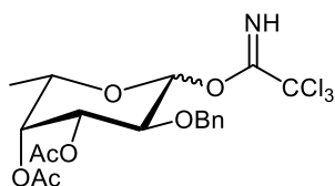
Fig. 1. Chemical structure of O -(2- O -benzyl-3,4-di- O -acetyl- \alpha/\beta -L-fucopyranosyl)-trichloroacetimidate.
