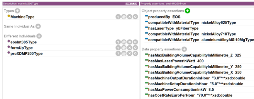
Fig. 4. Individual of Machine Type (EOSM290)
