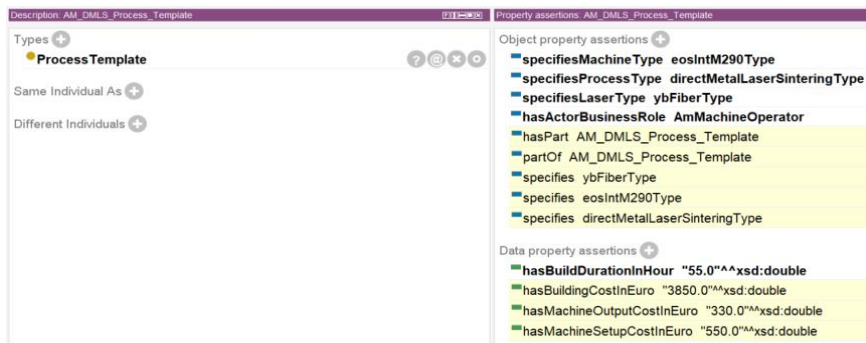
Fig. 3. Individual of AM Process Template (DMLS)
