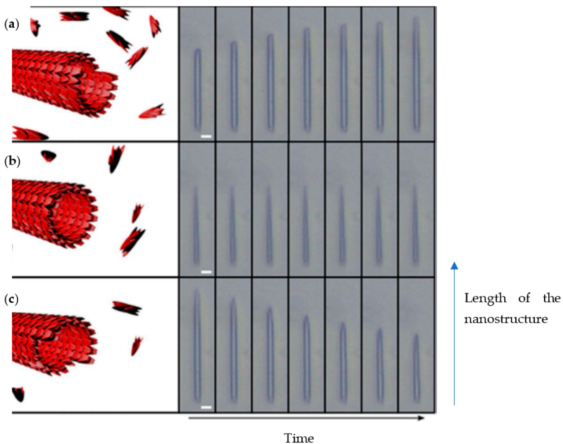
Figure 4. Elongation or shortening of FF nanotubes depending on monomer concentration in microfluidic platform. (a) supercritical concentration, (b) critical concentration, (c) subcritical concentration. Adapted with permission from Reference [33].
