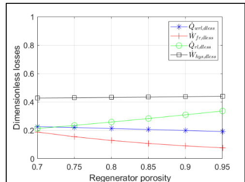
Figure 15. Variation of main losses with regenerator porosity
