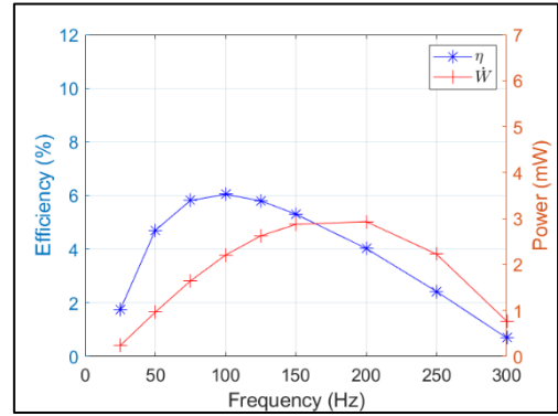
Figure 8. Variation of efficiency and power with frequency
