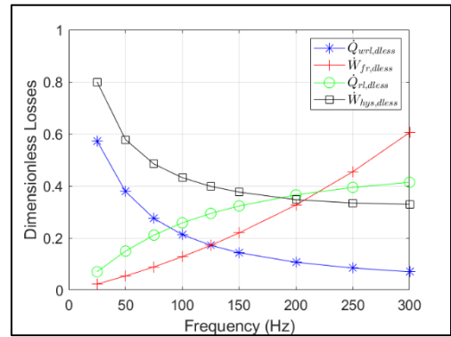
Figure 9. Variation of main losses with frequency
