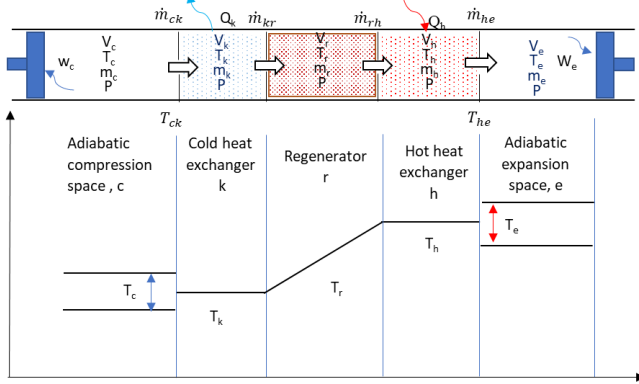
Figure 5. Adiabatic model
