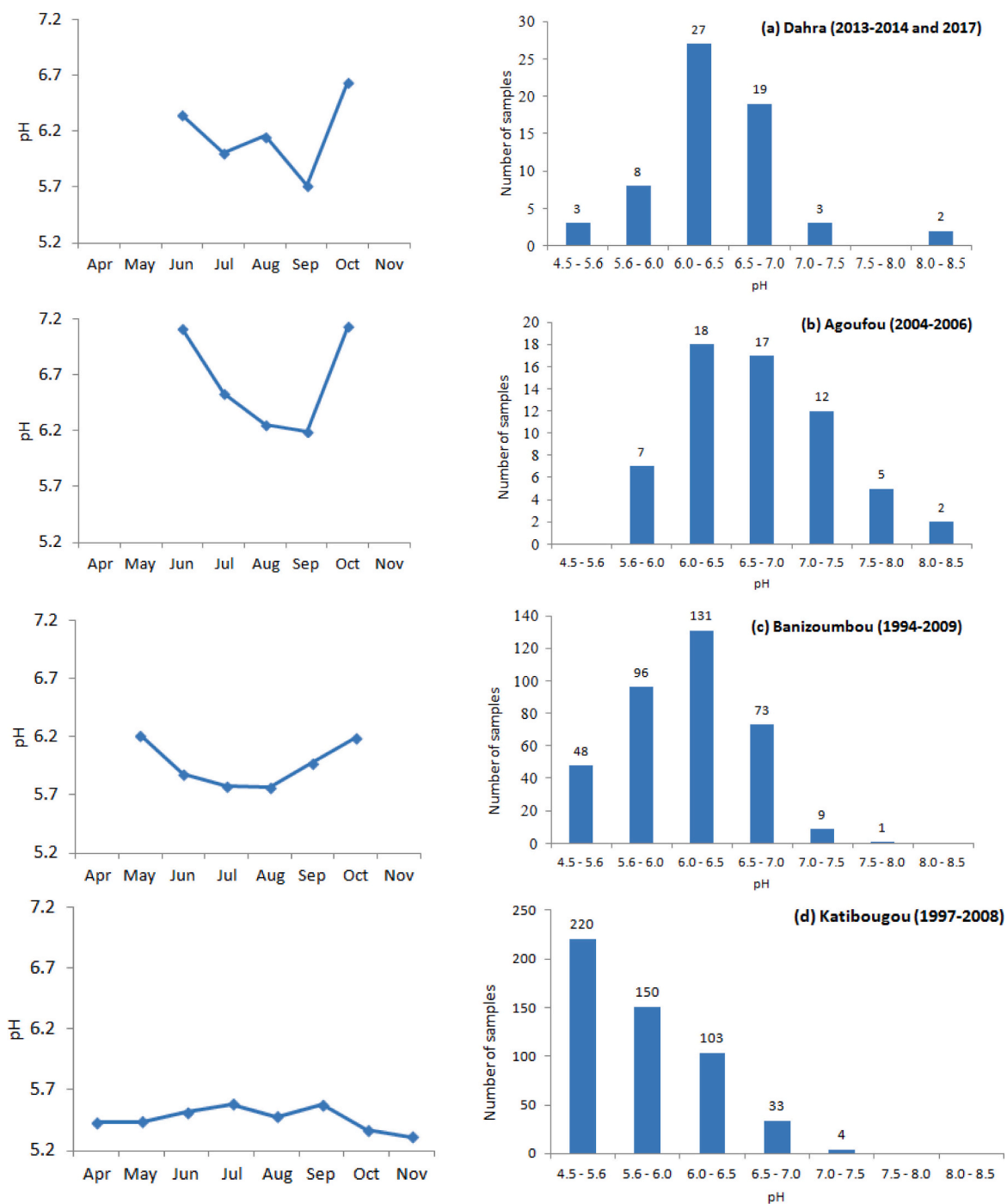
Fig. 5. Left: Temporal variation of pH in rainwater and Right: frequency distribution of pH values at the four Sahelian sites.
