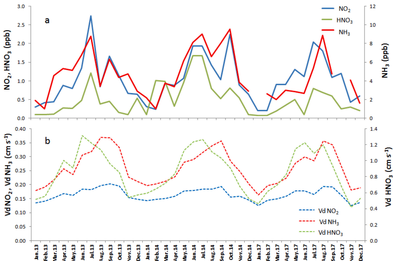
Fig. 6. (a) Monthly average concentrations of \text{NO}_2 , \text{NH}_3 and \text{HNO}_3 (ppb) measured by passive samplers at Dahra site and (b) deposition velocities for \text{NO}_2 , \text{NH}_3 and \text{HNO}_3 ( \text{cm s}^{-1} ) simulated with Zhang et al. (2003, 2010) model for years 2013, 2014, 2017.
