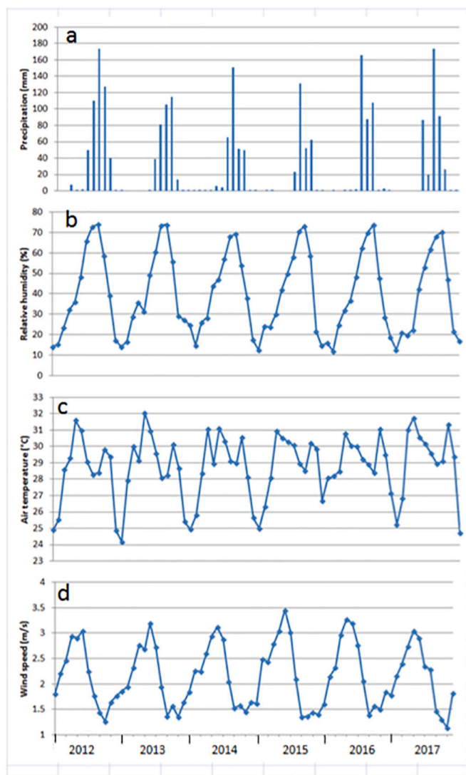
Fig. 2. (a) Monthly precipitation (mm), (b) relative humidity (%), (c) air temperature at 2 m ( ^{\circ}\text{C} ), and (d) wind speed at 2 m ( \text{m s}^{-1} ) at Dahra from 2012 to 2017. In (d) black vertical dashes correspond to the months of January for each year.
