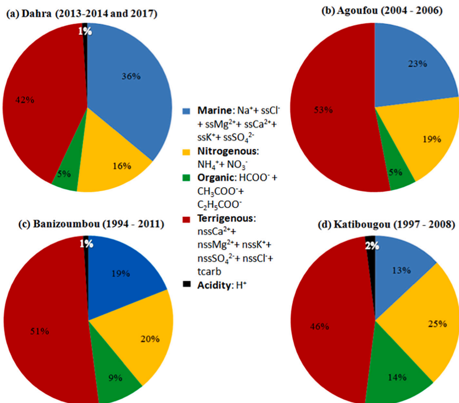
Fig. 3. (a-d): Estimation of the marine, nitrogenous, organic, acidity and terrigenous contributions to the rain chemical content measured at four Sahelian dry savanna sites of the INDAAF network.
