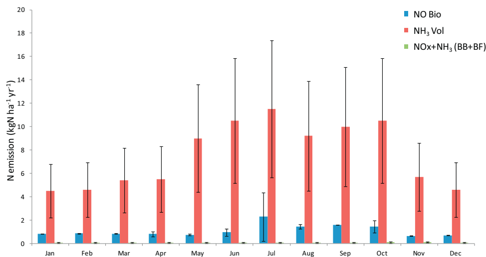
Fig. 7. Mean monthly distribution of nitrogen compound emissions in kgN ha -1 yr -1 , BB = Biomass Burning, BF= BioFuel, Vol. = Volatilization, NO Bio = Biogenic NO flux. Error bars indicate the standard deviation. These emissions are based on estimations for the period 2002–2007.
