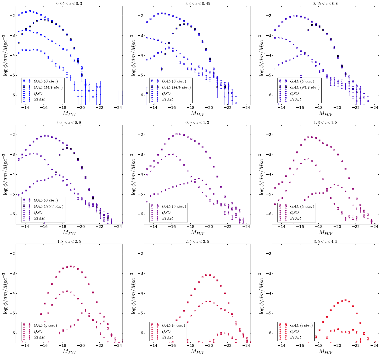
Figure C1. FUV LF of the different types of sources identified in our analysis: galaxies (GAL), quasars (QSO), and stars. The very bright end is mostly populated by stars and QSOs, which confirms that the deviation of the bright end of galaxy FUV LF from a pure Schechter form is likely to be due to contamination from stars and QSOs.
