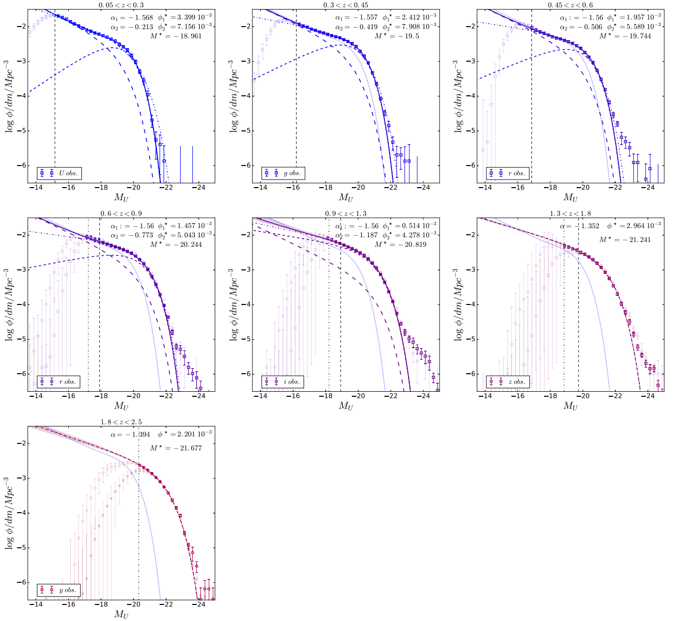
Figure 5. U-band LF measured at redshift 0.05 < z \leq 0.3 , 0.3 < z \leq 0.45 , 0.45 < z \leq 0.6 , 0.6 < z \leq 0.9 , 0.9 < z \leq 1.3 , 1.3 < z \leq 1.8 , and 1.8 < z \leq 2.5 . Similarly to Figs 3 and 4, at 0.6 < z < 1.8 , the faint end of the LF comes from our ultra-deep layer (open circles), and at 1.8 < z < 2.5 , the whole LF is based on the ultra-deep layer. In each panel, the solid line and associated envelop show our best Schechter fit and corresponding 1\sigma uncertainty. At z < 1.3 , both single-Schechter (dash-dotted lines) and double-Schechter (solid lines and associated envelops) functions are shown (the two components of the double-Schechter function are shown with dashed lines). At 0.45 < z < 1.3 , the faint-end slope of the double-Schechter function was set to \alpha_1 = -1.56 . At 1.3 < z < 2.5 , only a single Schechter was considered (see the text). Vertical dashed and dash-dotted lines show, respectively, the location of the deep and ultra-deep layer completeness limits (see Table 2).
