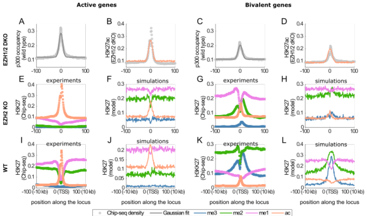
Figure 4: Predictions of H3K27 modifications for active and bivalent genes. (A,C) Average p300 occupancy in WT around active (A) and bivalent (C) genes. (B,D) Predictions of the average H3K27ac profile in EZH1/2 DKO cells for active (B) and bivalent (D) genes. (E-L) Experimental (E,G,I,K) and
