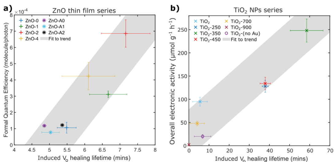
Figure 2. Calculated induced V_O healing lifetimes determined through PIERS analysis against measures of photocatalytic activity of a) a series of ZnO thin films and b) a series of TiO_2 NPs. The photoinduced V_O healing lifetime was calculated from SERS and PIERS average relative enhancements following the method previously described. 42 The photocatalytic activity of ZnO films was measured in terms of formal quantum efficiency for the degradation of stearic acid molecules. The photocatalytic activity of TiO_2 NPs was measured in terms of overall electronic activity, i.e., the mass- and time-normalized number of moles of electrons involved in the CO_2/H_2O to CH_4/H_2 reaction.
