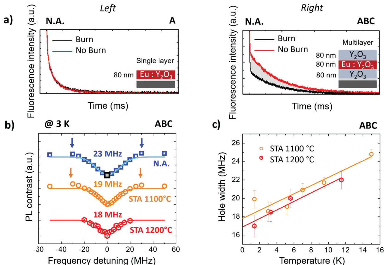
Fig. 7 SHB experiment at 3 K for A and ABC samples STA annealed for 2 h at various temperatures in air. (a) PL decay of the ^5\text{D}_0 \rightarrow ^7\text{F}_2 transition of Eu following the probe pulse used for the as deposited A (left) and ABC (right) samples. A strong PL decrease is only visible for the ABC sample the contrast of which is highlighted in grey and corresponding to the grey square in (b). (b) PL contrast as a function of central frequency detuning revealing a spectral hole in the ABC sample as-grown and after STA annealing. Anti-holes are also visible beside the hole central position (blue and orange arrows). Full lines are Lorentzian fits of the experimental data. (c) Hole width \Gamma_{\text{hole}} variation with temperature showing a linear trend.
