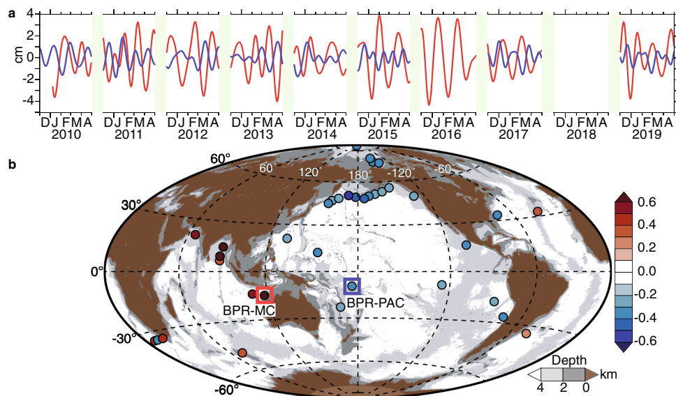
Fig. 3 See-saw in the bottom pressure recorders. a The plot of intraseasonal equivalent water depth at the BPR-MC (solid red; 117.94°E, 15.02°S, 5664 m) and the BPR-PAC (solid blue; 176.32°E, 9.517°S, 4921 m) during each December–April from 2009 to 2019. b Correlation (>90% significance; see methods section) of intraseasonal equivalent water depth from bottom pressure recorders across the globe with respect to the intraseasonal equivalent water depth at the BPR-MC (red box). All other bottom pressure recorders are marked as solid circles. The blue square box is used to mark BPR-PAC. The background color shades represent the bathymetry. The number of bottom pressure recorders analyzed in the Indian Ocean, Pacific Ocean, Atlantic Ocean, and the Arctic Ocean are 8, 45, 23, and 6, respectively.
