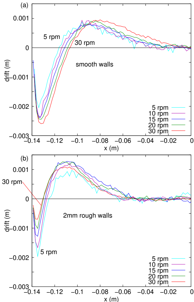
FIG. 9. Drift measured along the length of the left half of a 28 cm ( L/2R = 2 ) tumbler for various rotation speeds (5 to 30 rpm, Fr = 0.002 to 0.070 ). The tumbler has (a) smooth walls or (b) 2 mm rough walls and is filled at 30%. See Fig. S3 in Supplemental Material for 14 cm long tumblers [47].
