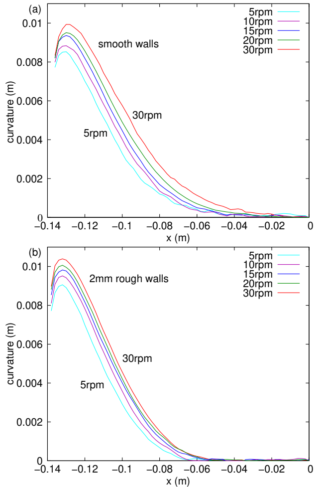
FIG. 10. Curvature measured along the 28 cm ( L/2R = 2 ) tumbler for various rotation speed (5 to 30 rpm, Fr = 0.002 to 0.070 ). The tumbler has (a) smooth walls or (b) 2 mm rough walls and is filled at 30%. Curvature for only the left half of the tumbler is shown. See Fig. S4 in Supplemental Material for 14 cm long tumblers [47].
