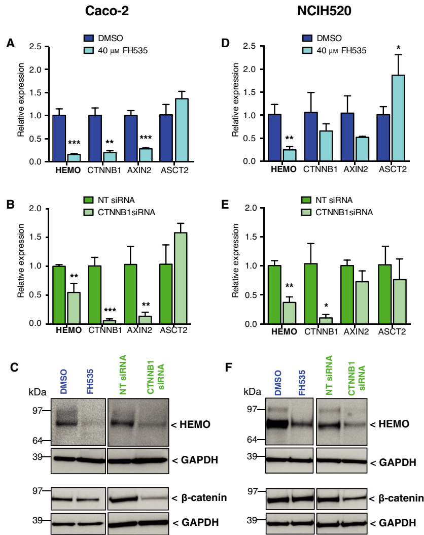
Fig. 7. HEMO expression decreases after Wnt/β-catenin inhibition in Caco-2 (A–C) and NCIH520 (D–F) cells. Inhibition was performed with 40 μM of FH535 (A: Caco-2, 72 h; D: NCIH520, 24 h) or by CTNNB1 silencing with siRNAs (B, E). Amount of mRNAs was normalized to housekeeping gene RPLP0 transcript level. Bar plots represent mean relative expression of three independent RT-qPCR experiments ± SD. (* P < 0.05; ** P < 0.01; *** P < 0.001, unpaired Student's t -test). Corresponding HEMO and β-catenin protein amount was assessed by western blot (C, F). GAPDH was measured as a control of cell lysate protein loading. NT: Non-targeting; ASCT2: neutral amino acid transporter.
