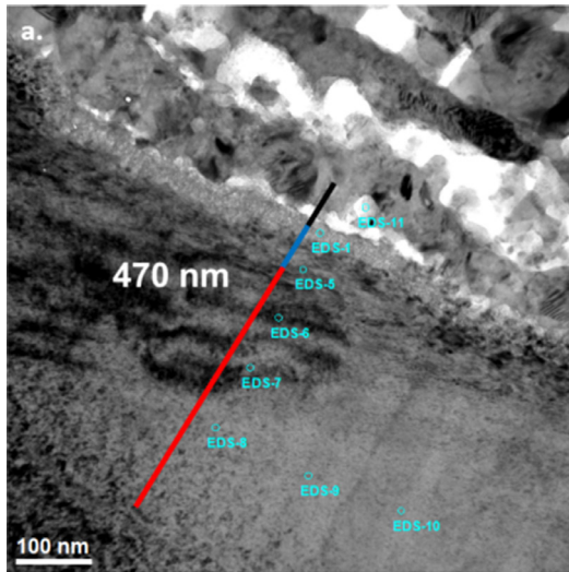
Fig. 13. (a) TEM observation and (b) relative EDS analysis of the alloy/oxide interface of the Ti6242S alloy oxidized at 650 °C for 1000 h in synthetic air.
