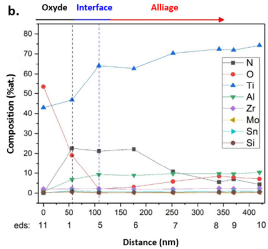
Fig. 13. (a) TEM observation and (b) relative EDS analysis of the alloy/oxide interface of the Ti6242S alloy oxidized at 650 °C for 1000 h in synthetic air.
