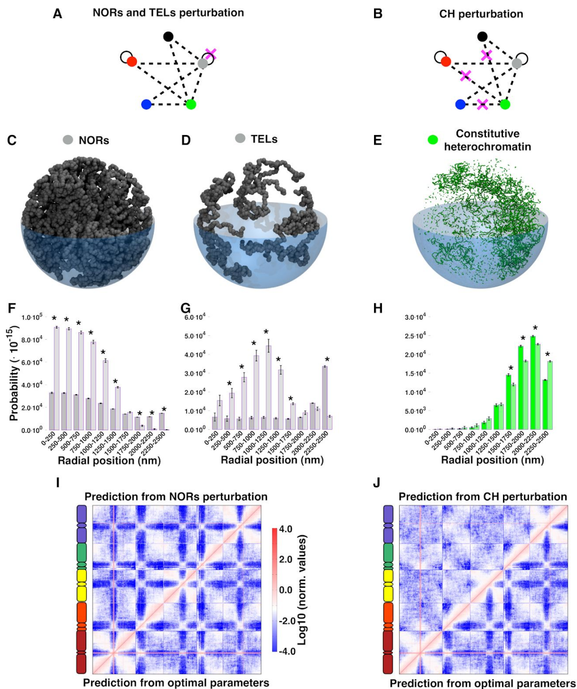
Figure 5. NORs and constitutive heterochromatin shape the A. thaliana nuclear organization. (A-B) Perturbed interaction networks. The interactions that are removed from the optimal case are crossed in magenta. (C-E) Illustrative snapshots for NOR (C) and telomeric (D) beads in the perturbed system shown in (A) . (E) As in (C, D) but for CH beads in the scenario shown in (B) . (G-H) Distributions of the radial positions of the 3kbp-regions in the perturbed systems (dark colour) compared to the
