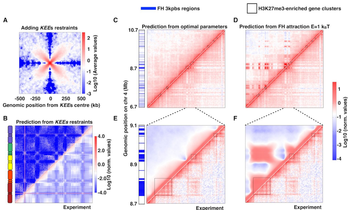
Figure 6. Plasticity of the optimal models in response to long-range and local interactions. (A) Average contact map of a 1Mbp-region around the KNOT Engaged Elements (KEEs) for the KEEs-restrained models. (B) Genome-wide contact maps in the KEEs-restrained case (top left triangle) and from experiments (bottom right triangle). (C-D) Predicted (top left triangles) vs experimental (bottom right triangles) contact maps at 30 kbp resolution in the chr4:6,700,000-10,700,000 bp region for the optimal set of parameters used in Figures 3 and 4 (C) or the optimal set complemented with strong self-attraction (1 k B T) between polycomb-like beads (D). (E-F) Zoomed views of (C-D) around the largest gene cluster (cluster 100 of Ref. (56)) (chr4:8,668,000-9,109,000 bp at 3 kb resolution). Black squares show the positions and extents of the gene clusters enriched in H3K27me3 mark (56). On the left of each map, blue lines indicate the positions of polycomb-like beads.
