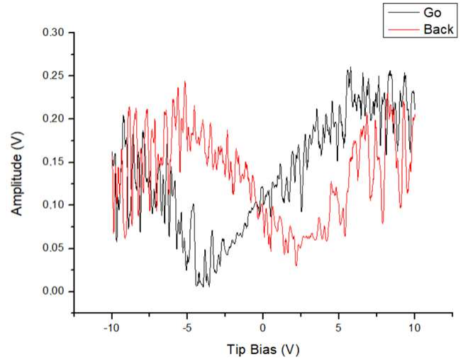
Fig. 5. The typical displacement versus tip voltage curve measured with a drive voltage of 5 \text{ V}
