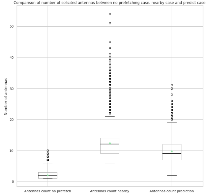
Figure 8: Activated antennas distribution for each scenario
