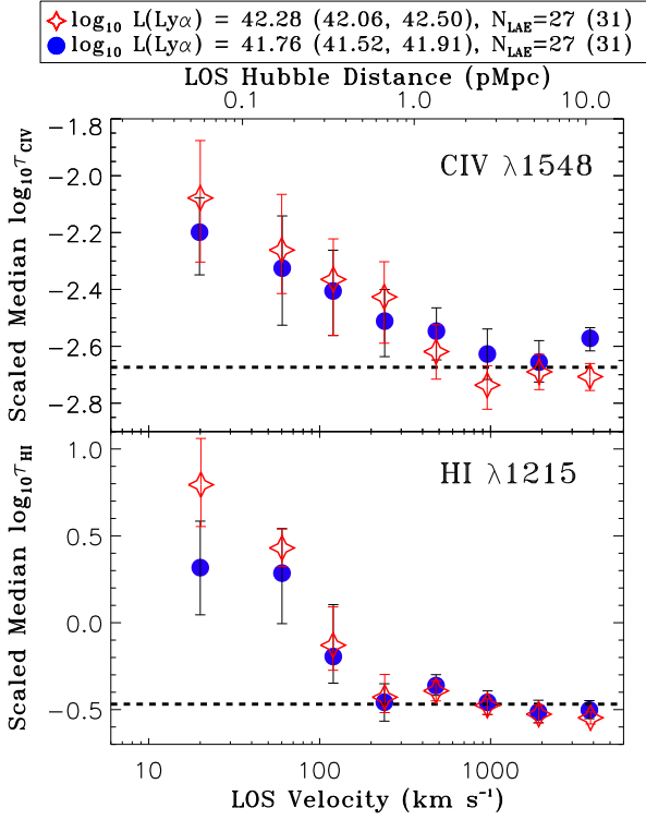
Figure 13. Similar to Fig. 9 but for two different luminosity bins ( \text{iso-}L(\text{Ly}\alpha)_{\text{low}} and \text{iso-}L(\text{Ly}\alpha)_{\text{high}} ). The median luminosities and 68 percentile ranges in the parentheses in the legends are for the LAEs contributing to the H I stack. The corresponding values for the CIV stack can be found in Table 3. No significant dependence on \text{Ly}\alpha line luminosity is seen for either H I or CIV absorption.
