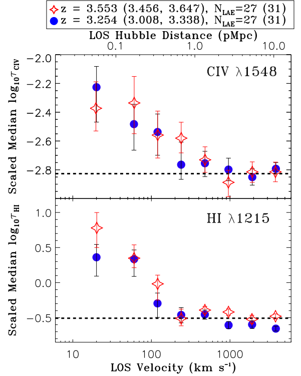
Figure 12. Similar to Fig. 9 but for two different redshift bins (iso- z_{\text{peak\_low}} and iso- z_{\text{peak\_high}} ). The median redshifts and 68 percentile ranges in the parentheses in the legends are for the LAEs contributing to the H I stack. The corresponding values for the C IV stack can be found in Table 3. No significant dependence on redshift is seen for either H I or C IV absorption.
