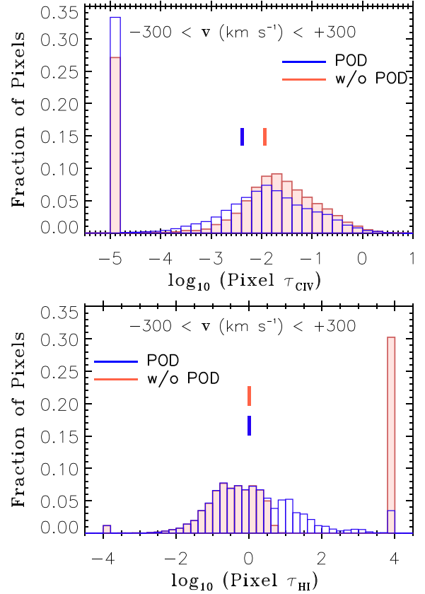
Figure 3. Histograms of pixel optical depths with and without POD recovery using PODPY. All pixels in the quasar spectra within \pm 300 \text{ km s}^{-1} of z_{\text{peak}} are used in these plots. There are 77 (92) LAEs contributing to the H I (C IV) pixel optical depth distribution in the bottom (top) panel. For H I, the pixels with very high and low optical depths ( >10^4 and <10^{-4} ) are flagged with flag values of 10^{+4} and 10^{-4} , respectively. For C IV, the pixels with \tau > 10^1 and \tau < 10^{-5} are flagged with flag values of 10^{+1} and 10^{-5} , respectively. The median values of the distributions are indicated by the vertical ticks with corresponding colours. The effect of the correction for saturation using higher order Lyman series lines by PODPY is evident from the bottom panel. The effects of the contamination correction and of rescaling the continua are apparent from the top panel.
