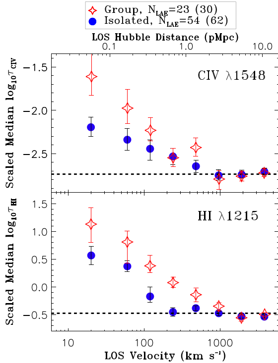
Figure 9. The median optical depth profiles of H I (bottom) and C IV (top) for the isolated (blue filled circles) and ‘group’ (red star symbols) subsamples. The top axis indicates the proper LOS distance at z = 3.3 corresponding to the velocity plotted along the bottom axis, assuming pure Hubble flow. To facilitate a proper comparison, the profiles of isolated and ‘group’ subsamples are taken to the same common baseline by linearly shifting one of the profiles by the difference in the background levels measured for the two profiles. A strong environmental dependence is seen for both H I and C IV with larger excess absorption around LAEs in ‘groups’.
