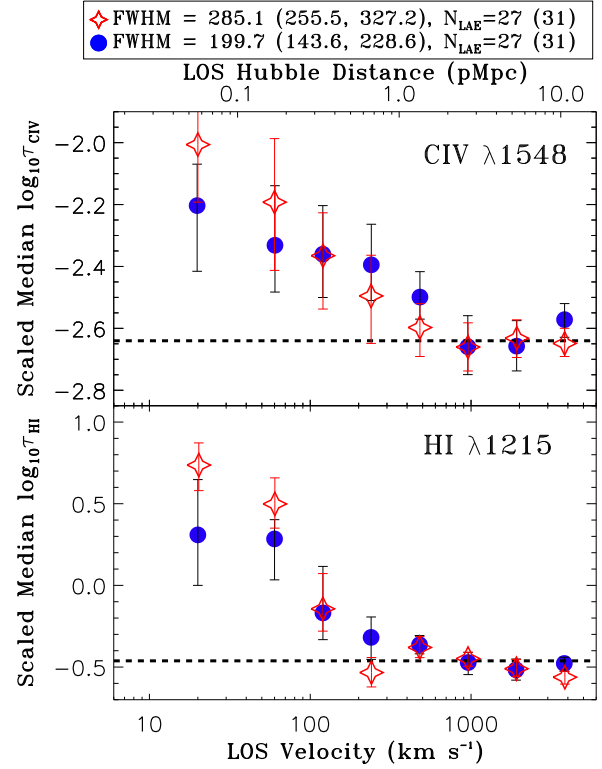
Figure 14. Similar to Fig. 9 but for two different FWHM bins ( \text{iso-FWHM}_{\text{low}} and \text{iso-FWHM}_{\text{high}} ). The median FWHM values and 68 percentile ranges in the parentheses in the legends are for the LAEs contributing to the H I stack. The corresponding values for the CIV stack can be found in Table 3. No significant dependence on FWHM of \text{Ly}\alpha emission is seen for either H I or CIV absorption.
