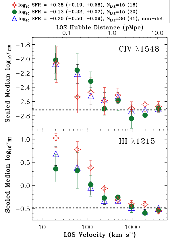
Figure 16. Similar to Fig. 9 but for three different SFR bins (all_SFR_non-det, blue; all_SFR_low, green; and all_SFR_high, red). The blue triangles represent the subsample of the UV-continuum-undetected objects. The median SFR values and 68 percentile ranges in the parentheses in the legends are for the LAEs contributing to the H I stack. The corresponding values for C IV stack can be found in Table 3. The H I profile is stronger and wider for the highest SFR bin, suggesting a strong SFR dependence. The noisier C IV profiles do not show any SFR dependence.
