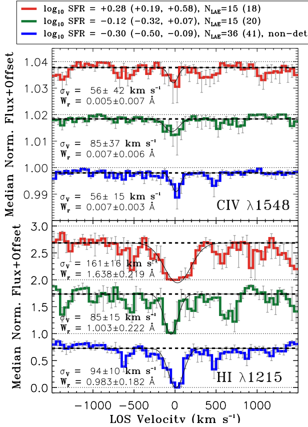
Figure 15. Similar to the right-hand panel of Fig. 8 but for three different SFR bins (all_SFR_non-det, blue; all_SFR_low, green; and all_SFR_high, red). The profiles in blue represent the subsample of the UV-continuum-undetected objects. The median SFR values and 68 percentile ranges in the parentheses in the legends are for the LAEs contributing to the H I stack. The corresponding values for C IV stack can be found in Table 3. The H I absorption shows a strong dependence on the SFR. The noisier C IV absorption profiles do not show any significant differences.
