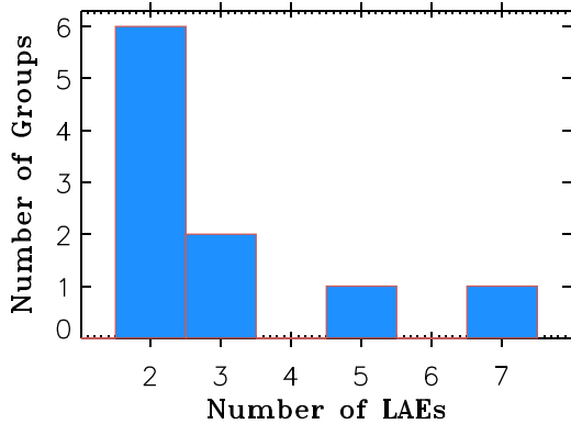
Figure 7. Histogram of the number of galaxies per group in the ‘group’ subsample. Most of the ‘groups’ in our sample consist of two detected LAEs.
