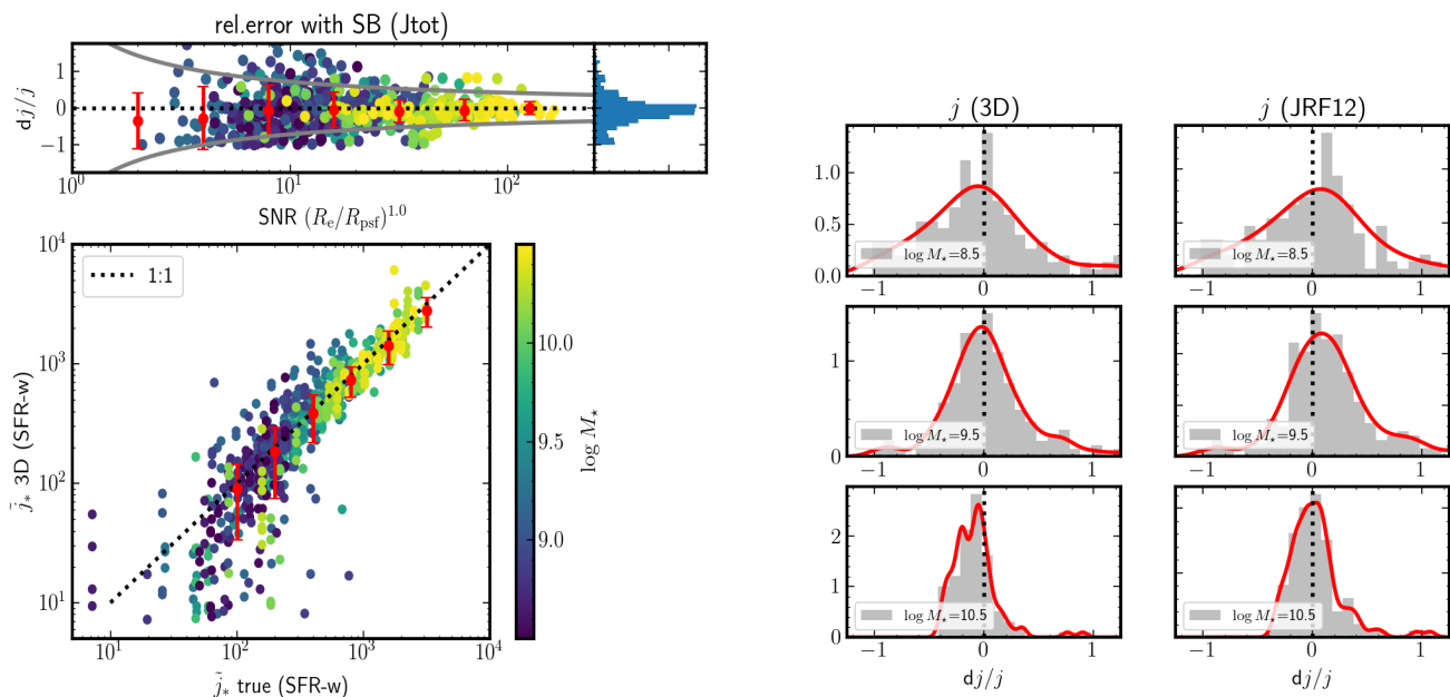
Fig. 6. Reliability of our sAM estimator. Left: The bottom panel shows the total SFR-weighted sAM, \tilde{j}_* (in \text{km s}^{-1} kpc), as a function of the true angular momentum (SFR-weighted) for the 790 mock galaxies. The top panel shows the relative error (\tilde{j}_* - j_{\text{true}})/j_{\text{true}} as a function of the effective S/N (see text) along with the histogram of d\tilde{j}_*/\tilde{j}_* . The points are colored according to the stellar mass in both panels. The red circles represent the median d\tilde{j}_*/\tilde{j}_* whose errorbar represent 1\sigma . Right: The relative error (d_j/j \equiv \tilde{j}_* - j_{\text{true}})/j_{\text{true}} for each mass bin of 1 dex centered on \log M_* = 8.5, 9.5, 10.5 , from top to bottom. The histograms are weighted by the errors. The left (right) panels show the distributions of d\tilde{j}_*/\tilde{j}_* , in three mass bins, resulting from the 3D method (the Eq. 3 approximation), respectively. The red solid line represents the continuous density estimation of the distributions using a Gaussian kernel with bandwidth of \sim 0.2 . This shows that, for massive galaxies ( M_* > 10^{10} M_\odot ), the Eq. 3 approximation is less biased, while for galaxies with M_* < 10^{10} M_\odot , the 3D method is less biased.
