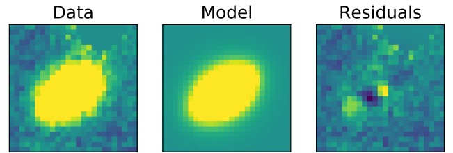
Figure A3. Comparison between data and GALFIT model for a broadband image ( r' ) of the main galaxy. All the data, the model, and the residuals (data-model) are scaled identically. The cutouts have a size of 5'' \times 5'' .
