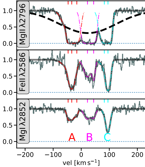
Figure 7. Absorption seen in the quasar UVES spectrum at the redshift of the main galaxy. Detected lines are transitions of MgII, MgI, and FeII, for each of which one transition is shown. The thin grey line are the observed UVES data, while the thick line is a model fit to the data. This model consists of the seven components at velocities as indicated on the top. Three main kinematic components (A, B, C) can be visually identified, the contributions of which to the model are indicated by the red, magenta, and cyan lines, respectively. The black dashed line in the MgII \lambda 2796 panel is the UVES spectrum artificially degraded to the resolution of MUSE at this wavelength.
