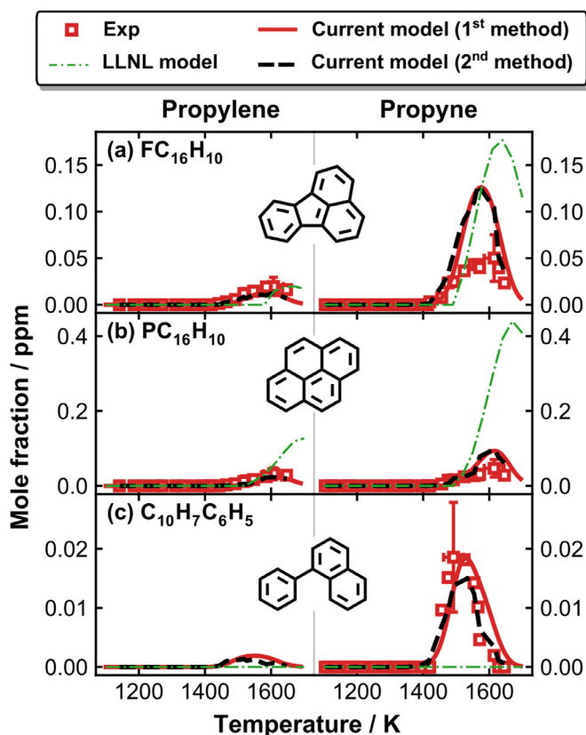
Fig. 18. Measured (symbols) and simulated (lines) fluoranthene ( FC_{16}H_{10} ), pyrene ( PC_{16}H_{10} ) and 1-phenyl-naphthalene ( C_{10}H_7C_6H_5 ) mole fraction profiles as a function of T_5 in propyne pyrolysis. Thick solid red lines: simulations using the current kinetic model with the constant p_5 of 20 bar and the nominal reaction time of 4 ms; thick dashed black lines: simulations using the current model with measured pressure profiles up to 10 ms; thin dot dashed green lines: simulations using the LLNL PAH model [64] with constant p_5 of 20 bar and the nominal reaction time of 4 ms. (For interpretation of the references to color in this figure legend, the reader is referred to the web version of this article.)
