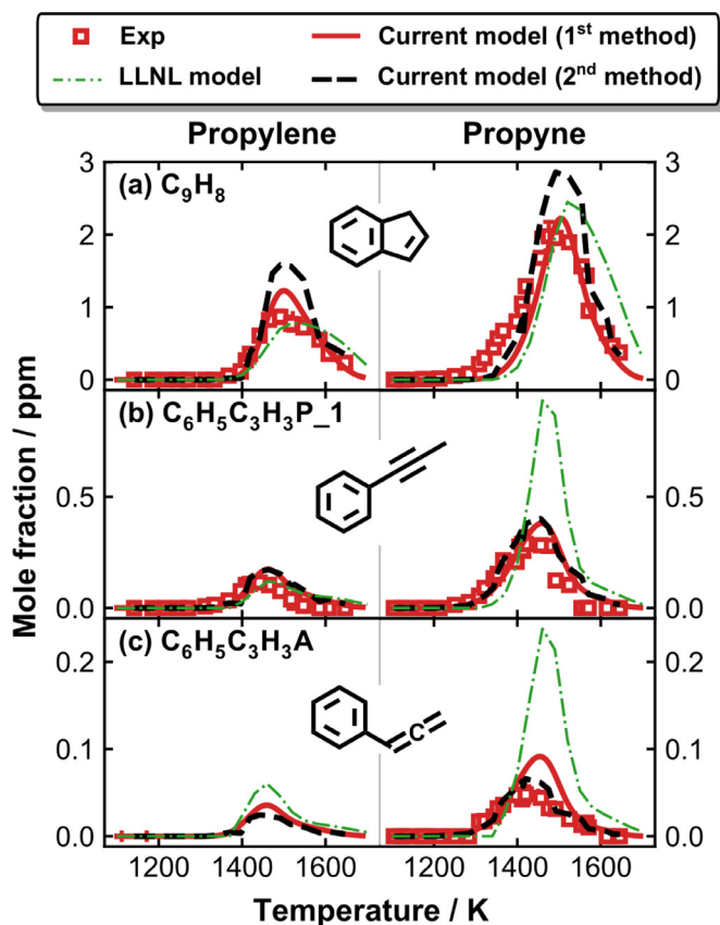
Fig. 13. Measured (symbols) and simulated (lines) mole fraction profiles for C_9H_8 isomers as a function of T_5 in propylene pyrolysis. Thick solid red lines: simulations using the current kinetic model with the constant p_5 of 20 bar and the nominal reaction time of 4 ms; thick dashed black lines: simulations using the current model with measured pressure profiles up to 10 ms; thin dot dashed green lines: simulations using the LLNL PAH model [64] with constant p_5 of 20 bar and the nominal reaction time of 4 ms.
