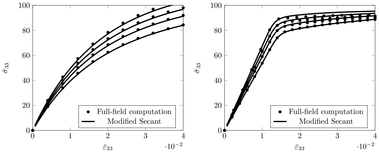
a. Linear elastoplastic case b. Elasto-viscoplastic case Figure 1. Macroscopic stress evolution with the prescribed macroscopic strain as predicted by the modified secant model and the full-field calculations as a function of defective inclusions. Material data are respectively given in table 1 and 2.
