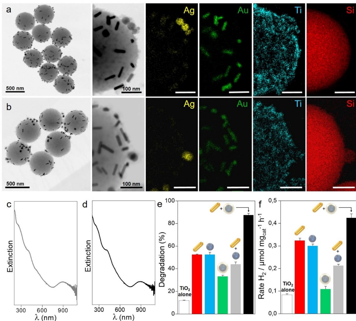
Figure 3. STEM images (bright field) and EDX mapping of the hybrid materials composed by (a) the assembly of Au NRs, Ag NPs and \text{TiO}_2 NPs and (b) by the assembly of Au NRs, Ag@ \text{SiO}_2 NPs and \text{TiO}_2 NPs onto the \text{SiO}_2 beads. (c, d) Extinction spectra of the hybrid nanostructures based on Au NRs + Ag NPs and Au NRs + Ag@ \text{SiO}_2 NPs, respectively. Comparison of the activity of the different hybrids synthesized in the present work in two different reactions: (e) photocatalytic degradation of RhB after 180 min of solar-simulated irradiation at 25 °C and (f) photocatalytic \text{H}_2 generation assisted by formic acid after 60 min of solar-simulated irradiation at 35 °C. Plasmonic components: 100 nmol/mg \text{SiO}_2 of Au NRs (red), 100 nmol/mg \text{SiO}_2 of Ag NPs (blue), 100 nmol/mg \text{SiO}_2 of Ag@ \text{SiO}_2 NPs (green), 100 nmol/mg \text{SiO}_2 of Au NRs + 100 nmol/mg \text{SiO}_2 of Ag NPs (grey); 100 nmol/mg \text{SiO}_2 of Au
