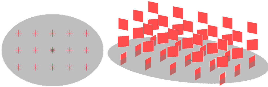
Figure 22: Lifting of the tangent planes AT(p) . In this case the tangent planes have the same dimension at every p . Left: The base of the fiber bundle. Right: The lifting of tangent vectors in a higher dimensional space (x, y, \theta) is a fiber bundle.
