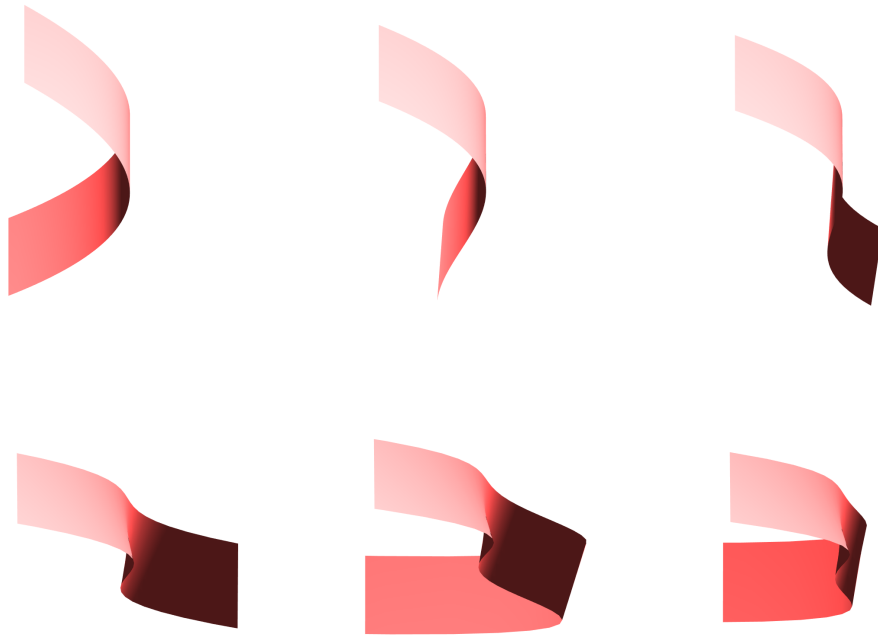
Figure 34: Evolution of Thom's elementary catastrophes with potential V_\tau = (1 - \tau)V_1 + \tau V_2 from the V_{fold} (first frame) to the V_{cusp} (4th frame) and to the V_{swallowtail} (last frame). The equilibrium manifold \frac{\partial V(x,p)}{\partial x} = 0 is visualised.
