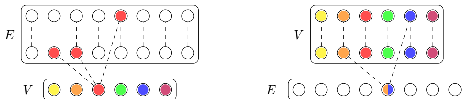
(a) Co-2-subdivision of subcubic graphs: edges are represented by an antimatching, vertices, by a clique.
