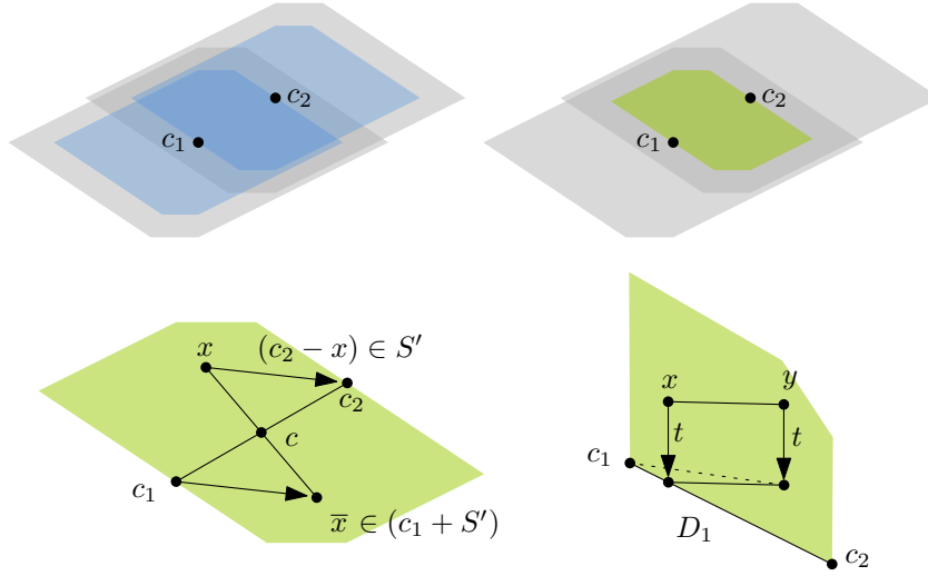
■ Figure 4 Top left: The gray sets are scaled about their center so that the center of one set is on the boundary of the other. Top right: the intersection D . Bottom left: Illustration of Lemma 12. Bottom right: Illustration of Lemma 14.
