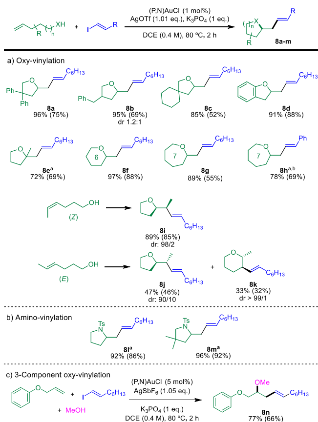
Scheme 5. Gold-catalyzed hetero-vinylation, scope of alkenols and N -tosyl alkenamines, as well as 3-component oxy-vinylation. Yields determined by ^1\text{H} NMR spectroscopy with dimethyl terephthalate as internal standard. Isolated yields in parentheses. a 5% (P,N)AuCl, 1.05 eq. AgOTf. b 25 °C, 16 h.
