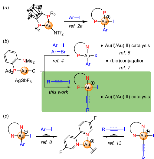
Figure 1. Ligand-enabled oxidative additions of C–I/C–Br bonds to gold.
