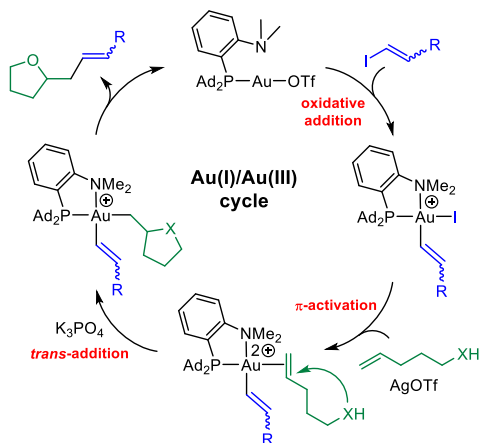
Figure 2. Catalytic cycle proposed to account for oxy-/amino-vinylation reactions catalyzed by the (P,N)Au(I) complex.
