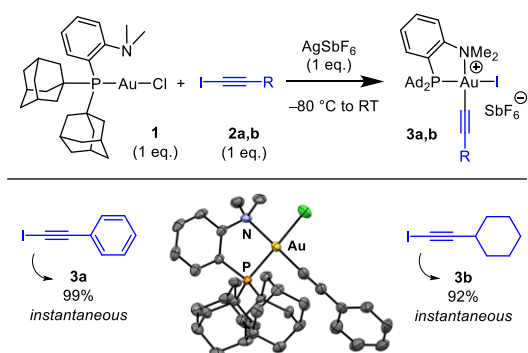
Scheme 1. Oxidative addition of alkynyl iodides to the (P,N)AuCl complex 1 . Reaction times and spectroscopic yields based on ^{31}\text{P} NMR. Molecular structure of the (P,N)Au(III) alkyne complex 3a (hydrogen atoms and counter anion omitted for clarity, ellipsoids shown at 50% probability).
