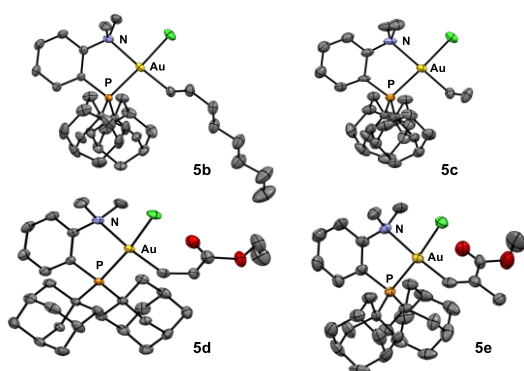
Scheme 2. Oxidative addition of vinyl iodides to the (P,N)AuCl complex 1 . Reaction times and spectroscopic yields based on ^{31}\text{P} NMR. Molecular structures of the (P,N)Au(III) vinyl complexes 5b-e (hydrogen atoms, counter anions and solvate molecules omitted for clarity, ellipsoids shown at 50% probability).
