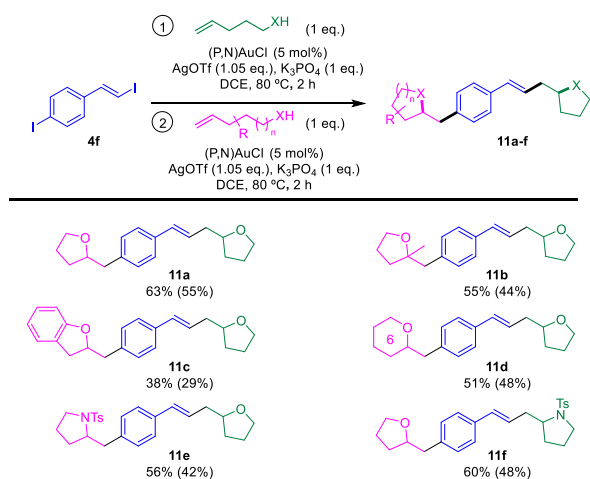
Scheme 7. Sequential gold-catalyzed hetero-vinylation/arylation transformations of the bifunctional substrate 4f . Yields over the two steps determined by 1 H NMR spectroscopy with dimethyl terephthalate as internal standard. Isolated yields in parentheses.
