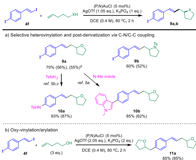
Scheme 6. Selective and sequential transformation of the bifunctional substrate 4f . Yields determined by ^1\text{H} NMR spectroscopy with dimethyl terephthalate as internal standard. Isolated yields in parentheses. a gram scale reaction (4 mmol).
