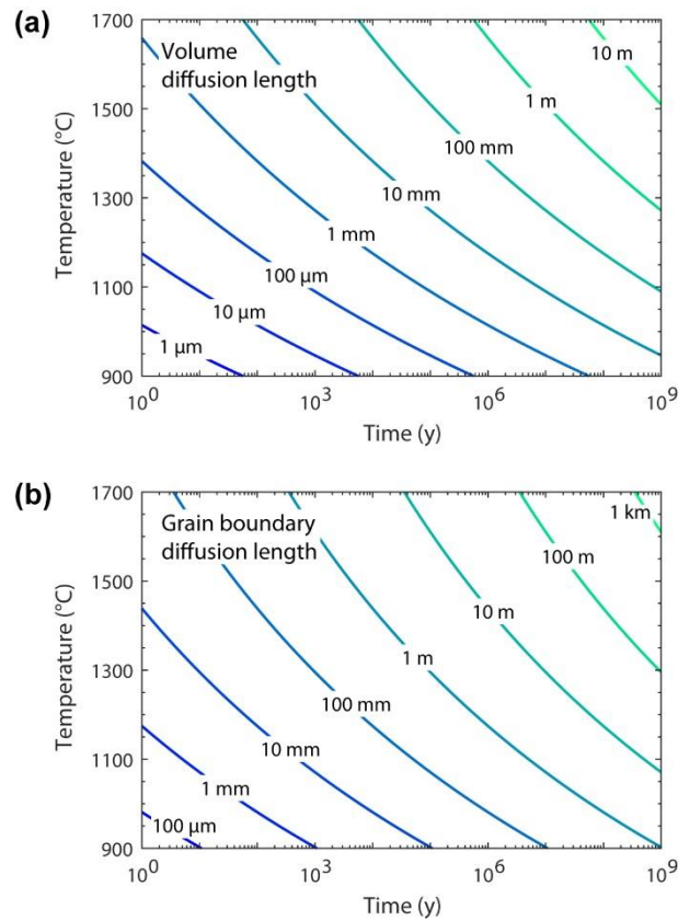
Fig. 11 Characteristic lengths of Mg diffusion in a volume and b grain boundary of Mg 2 SiO 4 at 1 atm. Lengths should be similar up to ~1 GPa, and decreased by factor up to ~3 up to 10 GPa at asthenosphere temperatures of 1300-1600°C. In iron- and hydrogen-bearing olivine, lengths should be increased by factor ~3-10 for both volume and grain boundary diffusion (see Text). Long-range transport of Mg in the mantle via solid-state, volume or grain boundary diffusion is precluded since km-scale is not reached even after 1 Gy at 1600°C. At short timescale of ~1 ky in the asthenosphere, volume diffusion rather acts at the scale of individual or adjacent grains and grain boundary diffusion may allow exchanges between a few hundred grains.
