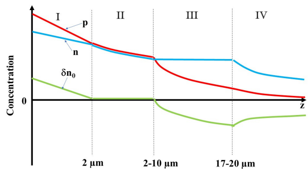
FIG. 9. Illustration of the spatial dependences of concentrations of photoelectrons n , photoholes p and of the relative concentration of intrinsic electrons \delta n_0 (see Sec. IV. A), for the various spatial phases defined in Fig. 2. The limits of these spatial phases depend on excitation power and their range of values is indicated. The amplitude of the Fermi sea redistribution \delta n_0 is negligible for an excitation power of 9 \mu\text{W} and increases with excitation power.
