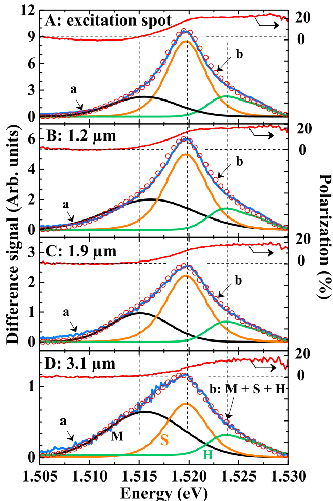
FIG. 4. Same as Fig. 3, but for the difference spectra. Also shown are the polarization spectra, defined as the ratio between difference signal and intensity. Note that, at large distance (Panel D), component S is still the dominant feature of the difference spectrum, while it has disappeared from the corresponding intensity spectrum.
