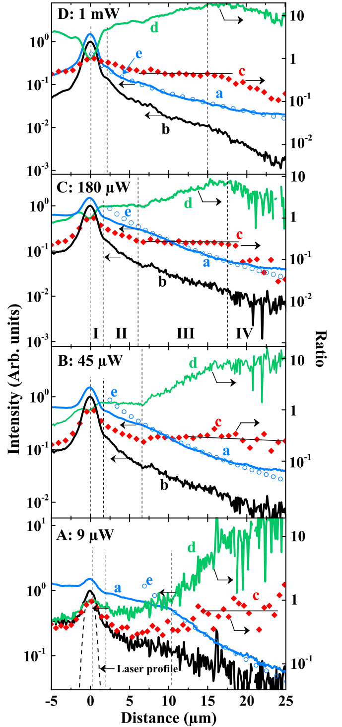
FIG. 7. Intensity spatial profiles of line M (1.515 eV, Curves a), of line H (1.527 eV, Curves b) for selected excitation powers of 9 \mu\text{W} (A), 45 \mu\text{W} (B), 180 \mu\text{W} (C) and 1 \text{ mW} (D). Each panel also shows the ratios \mathcal{C} (Curves c) and \mathcal{B} (Curves d), given by Eq. 13 and Eq. 12, respectively. Curves e are fits of Curve a using Eq. 14, describing ballistic hole transport over the fluctuations.
