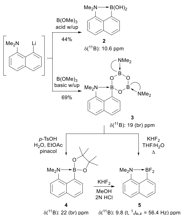
Scheme 6 Synthesis of the boronic acid 2 and boroxine 3 , subsequent reactivity at boron.
