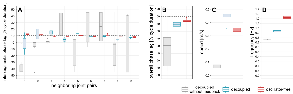
Fig. 5. Performance results of robot experiments in the decoupled and oscillator-free configurations. The decoupled configuration with and without feedback were each tested in n=6 experiments at an intrinsic frequency of 0.75 Hz. The oscillator-free configuration was tested in n=11 experiments and a central overall phase lag of 100 % (cycle duration). The oscillator phases were randomly initialized in all experiments. The performance metrics in (A) to (D) are described in Materials and Methods . The horizontal lines indicate the median. Box limits are the upper and lower quartiles and the whiskers show the values within a 1.5 x interquartile distance from the upper and lower quartiles, respectively. Outliers are represented as dots. Note that in (A), the intersegmental phase lag at the first joint for the decoupled configuration is not strictly positive. The dynamics of this joint would need more time to converge, however we were limited by the size of the swimming pool.
