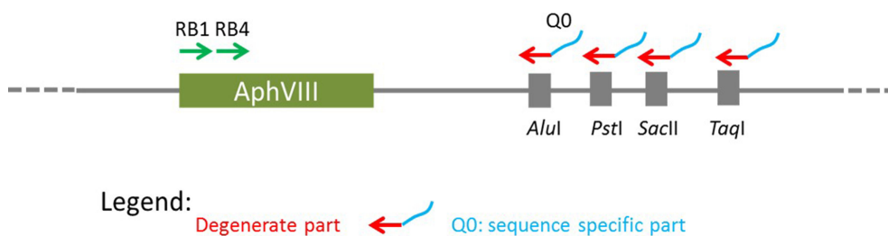
Figure 1. Outline of the principals for RESDA PCR. This schematic is adapted from González-Ballester et al. , 2005.
