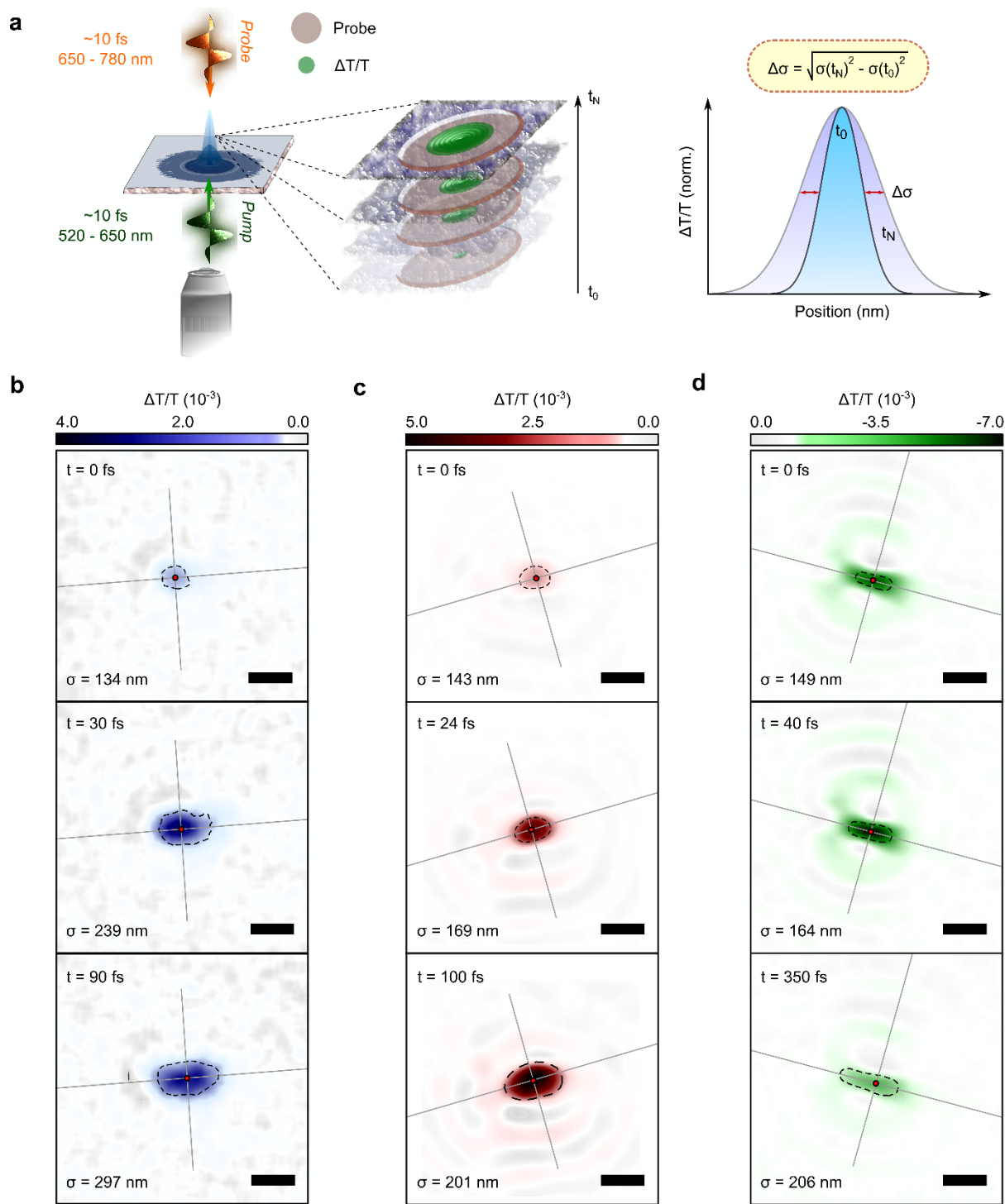
Figure 3: Femtosecond transient absorption microscopy of organic nanostructures. a. Schematic of fs-TAM. A diffraction limited pump pulse (green) is focused onto the sample by a high numerical aperture microscope objective. A probe pulse (yellow) is focussed from the top onto the sample in the wide-field. The transmitted probe is collected by the objective and imaged onto a digital camera (Supplementary Methods). Comparison of the spatial extent of the signal (stack) at different time delays allows us to dynamically track changes in the population with \sim 10 nm precision (right hand graph). b-
