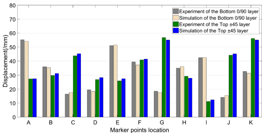
Fig. 14 Tetrahedral forming material draw-in comparison between simulation and experiment
