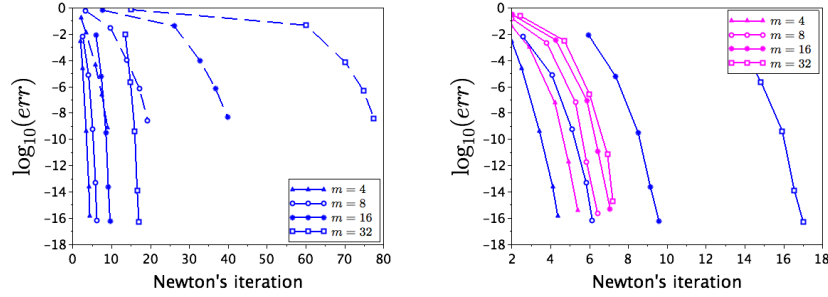
Fig. 1 Relative error err_{m,\varepsilon}^* as the function of the average number of Newton's iterations per time step. Left: for v -formulation (solid blue) and u -formulation (dashed blue). Right: for v -formulation (blue) and \tau -formulation (magenta).
